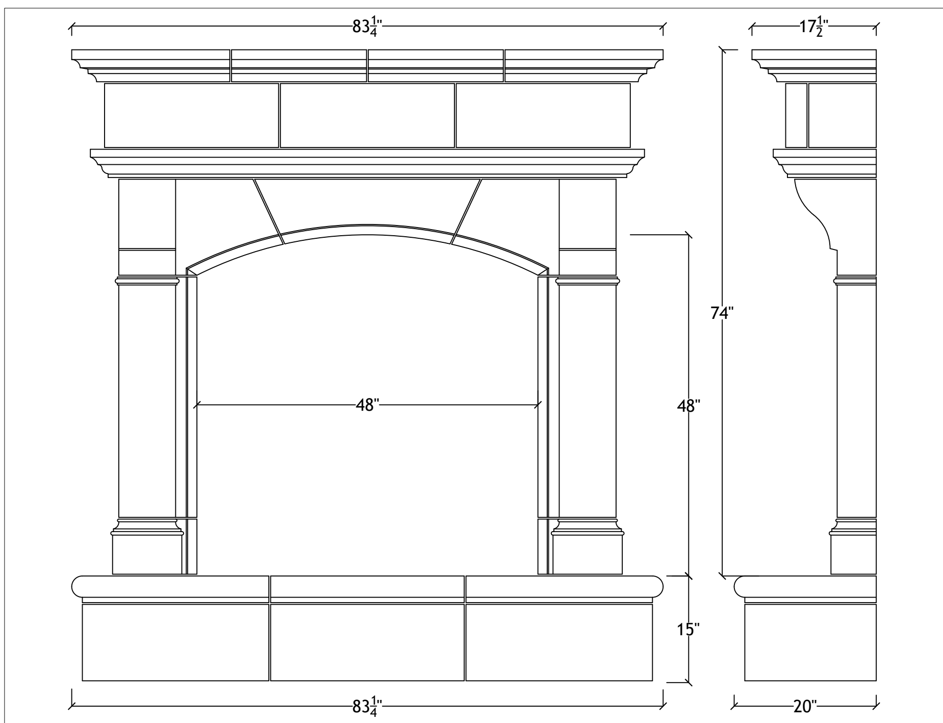
48" Normandy with raised bullnosed hearth
