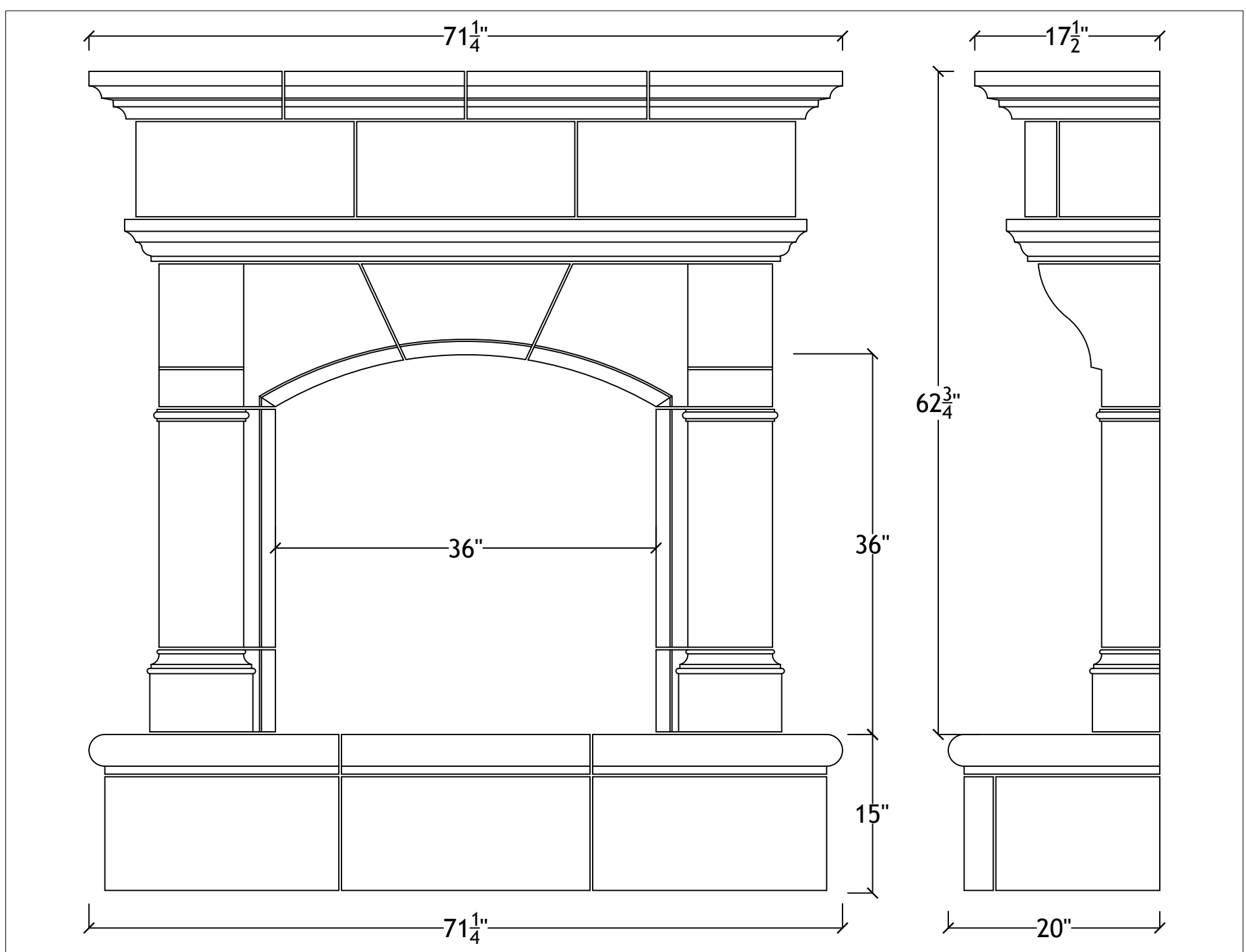
36" Normandy with raised bullnosed hearth
