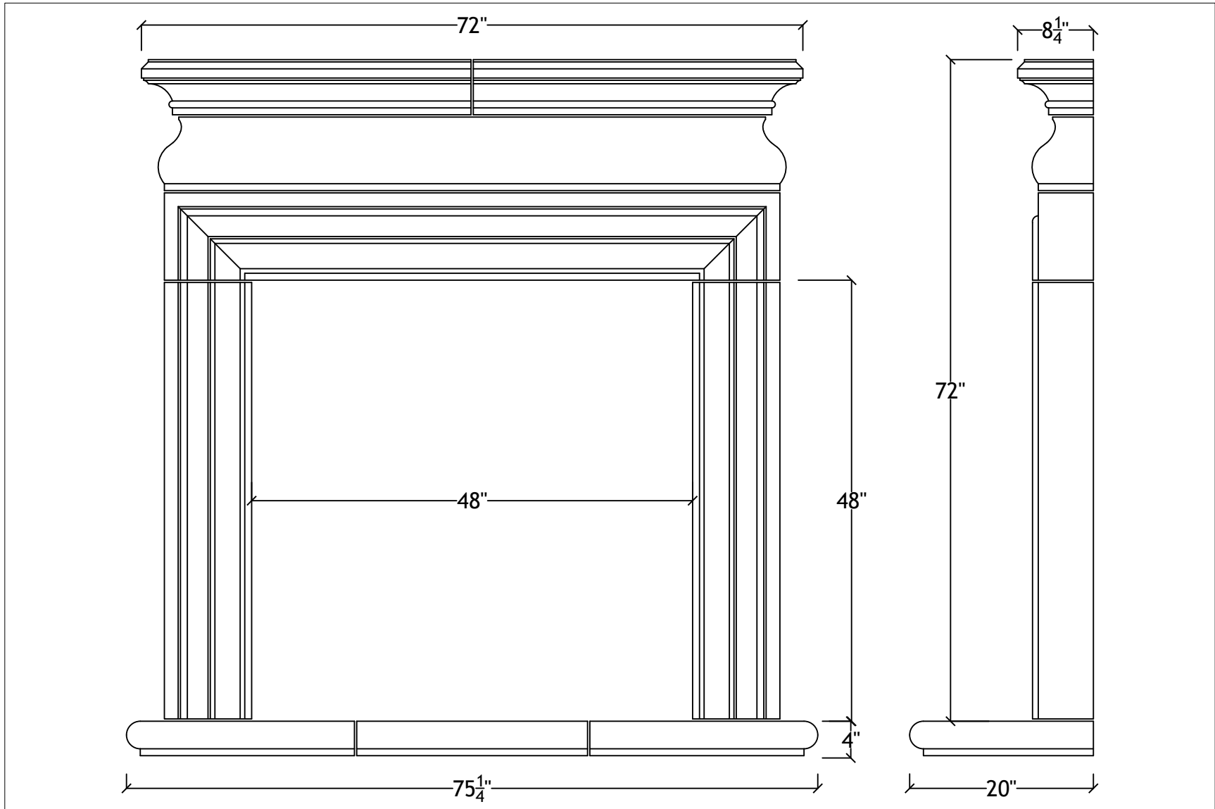
48" Newcastle with bullnosed hearth
