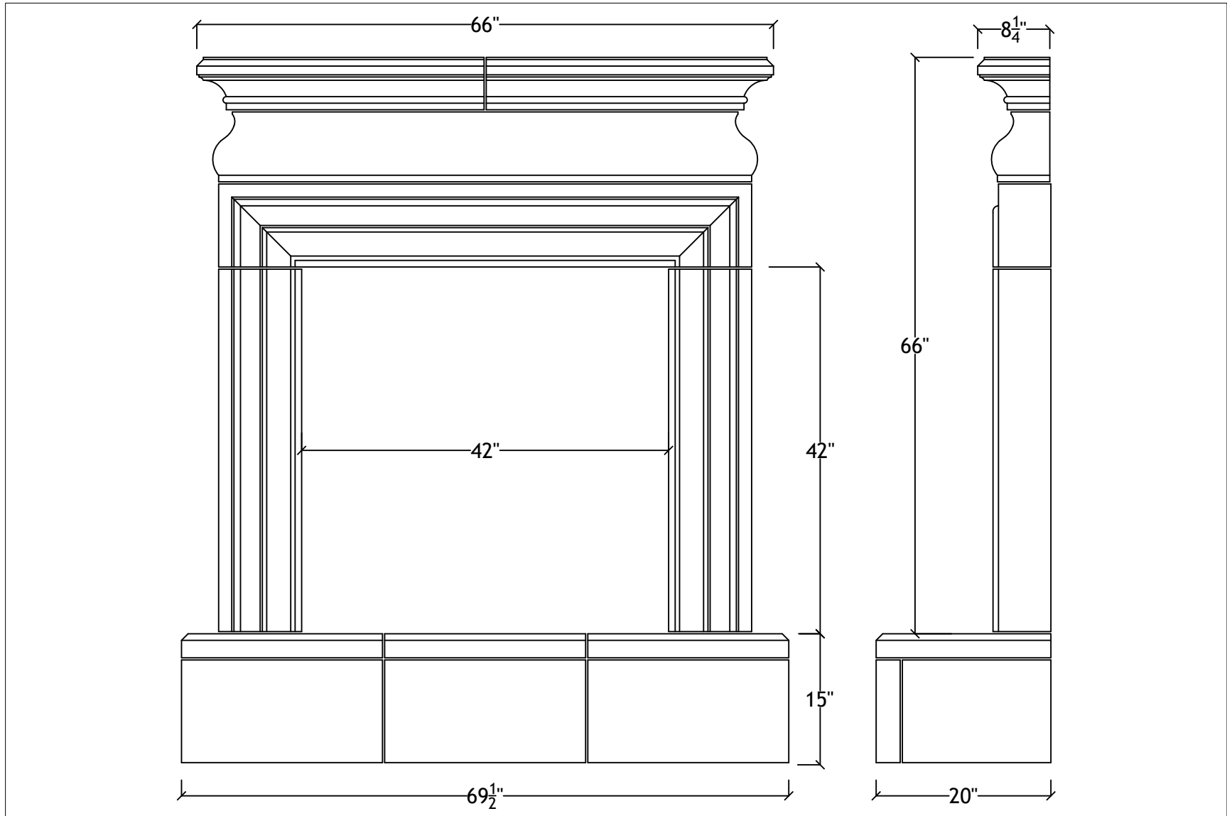
42" Newcastle with raised hearth
