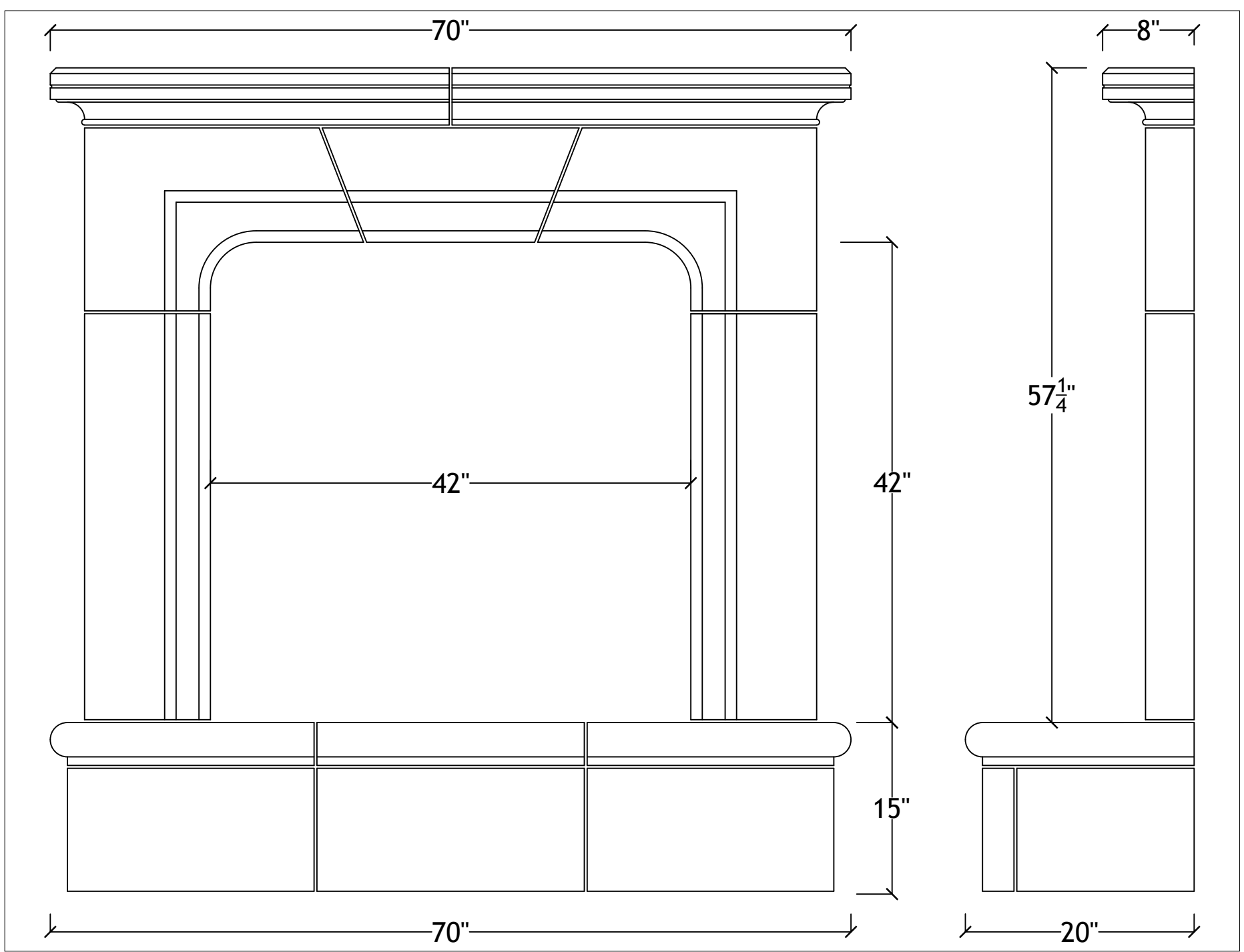
42" Montgomery with raised bullnosed hearth
