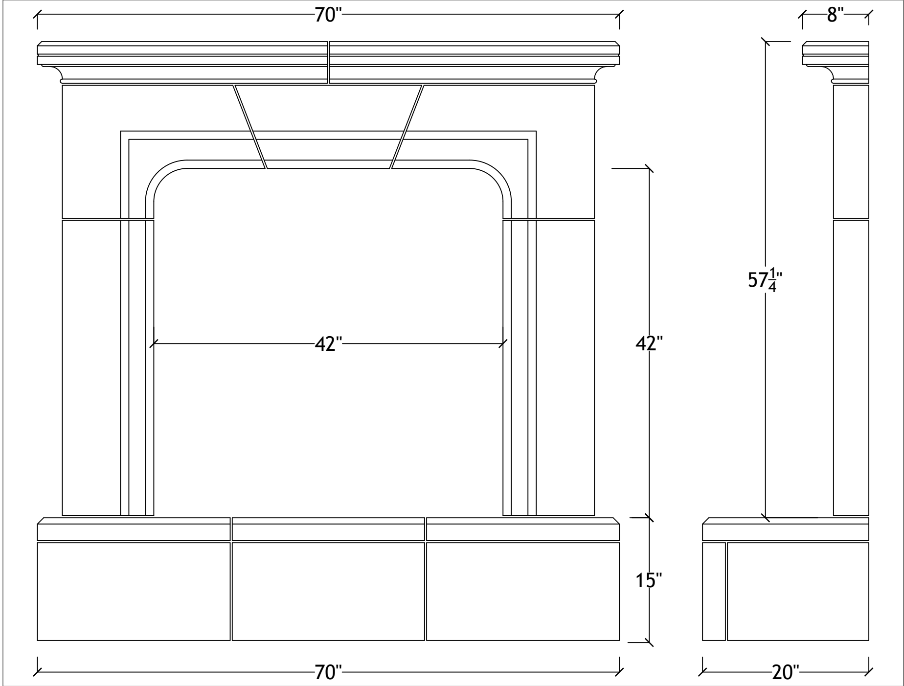
42" Montgomery with raised hearth
