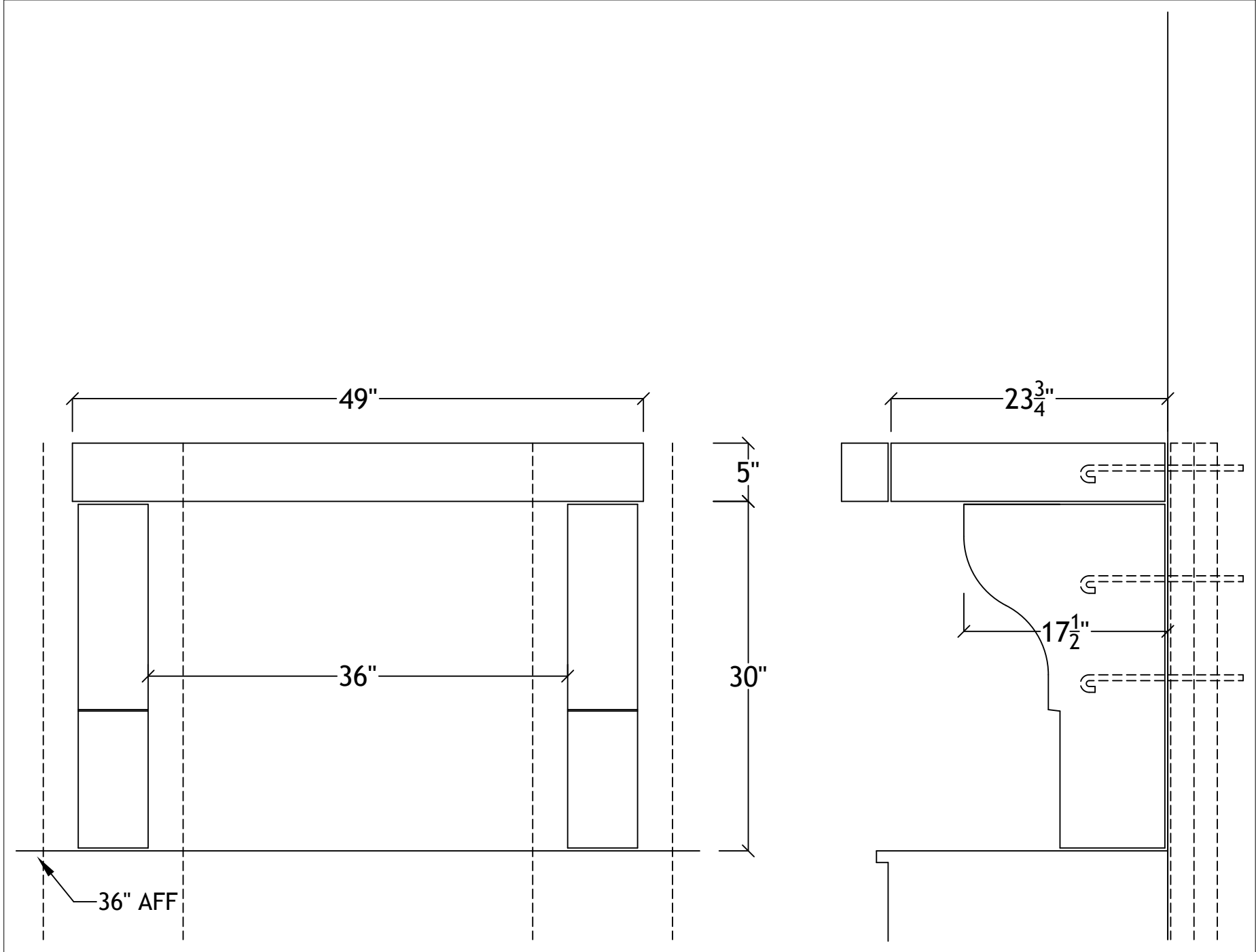
36" Modern Range Hood
