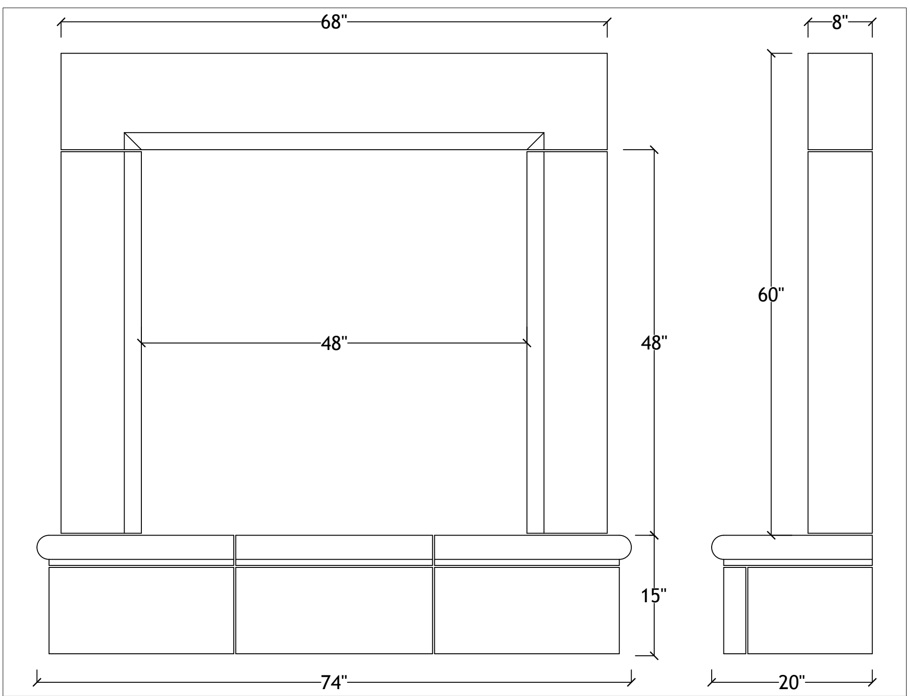
48" Manhattan with raised bullnosed hearth
