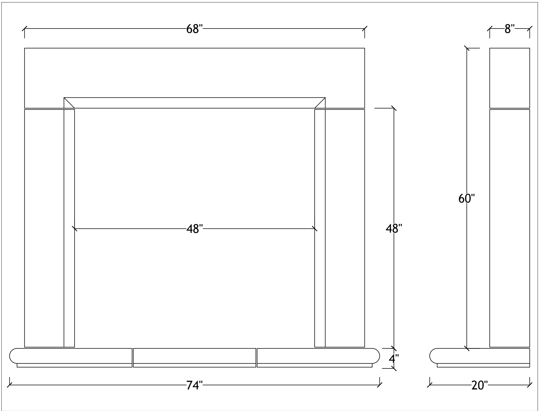
A 48" Manhattan with bullnosed hearth
