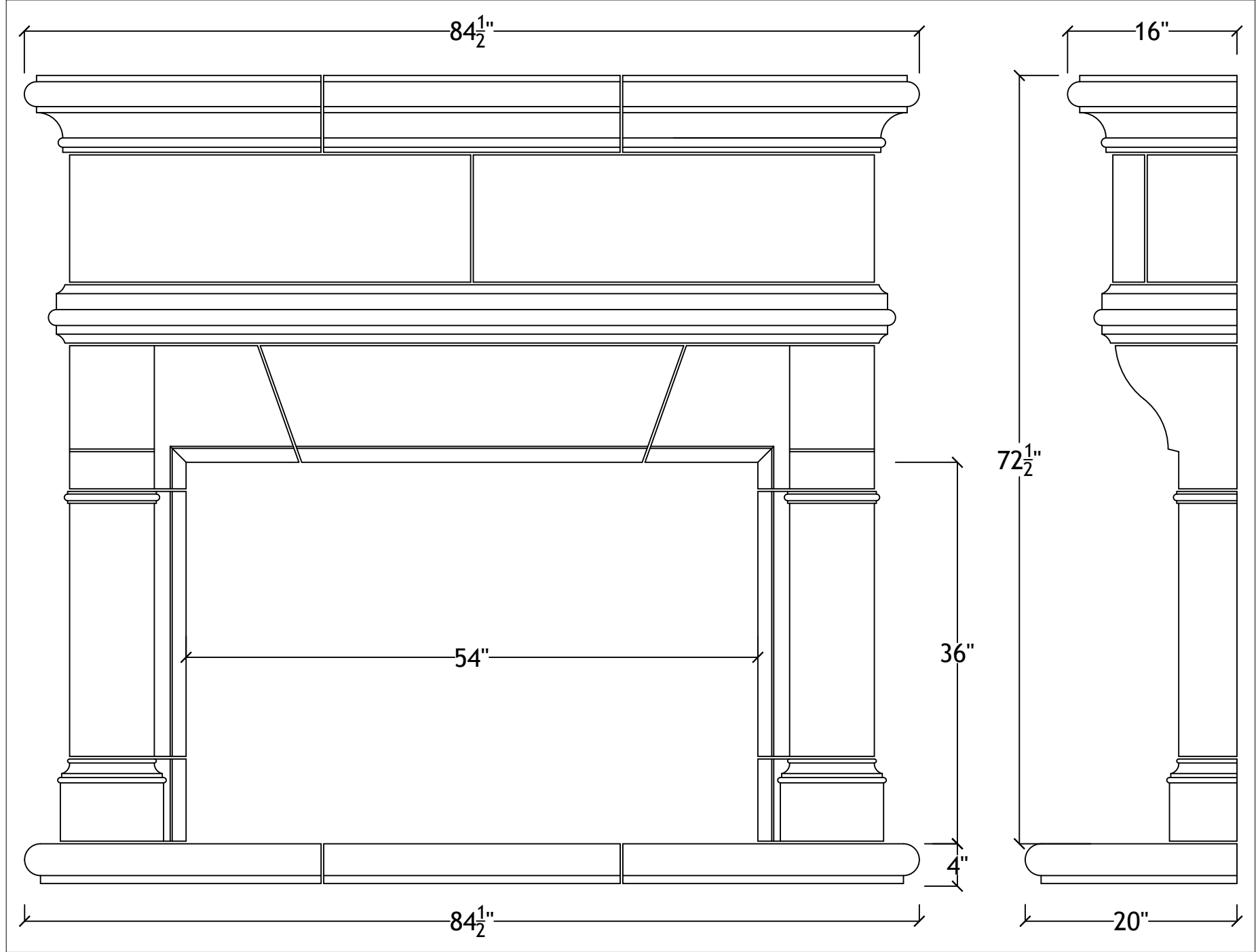
54" Mandalay with bullnosed hearth
