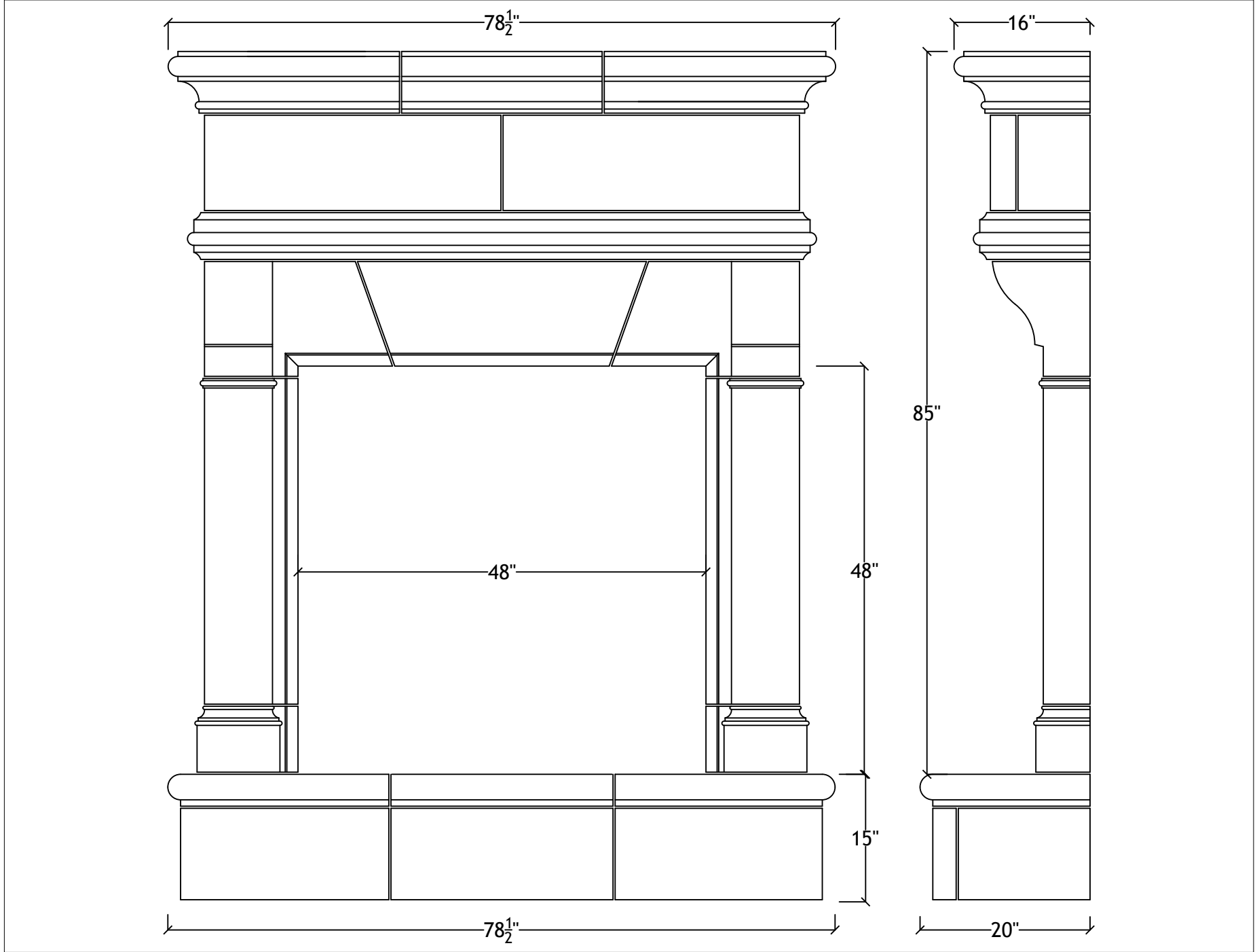
48" Mandalay with raised bullnosed hearth
