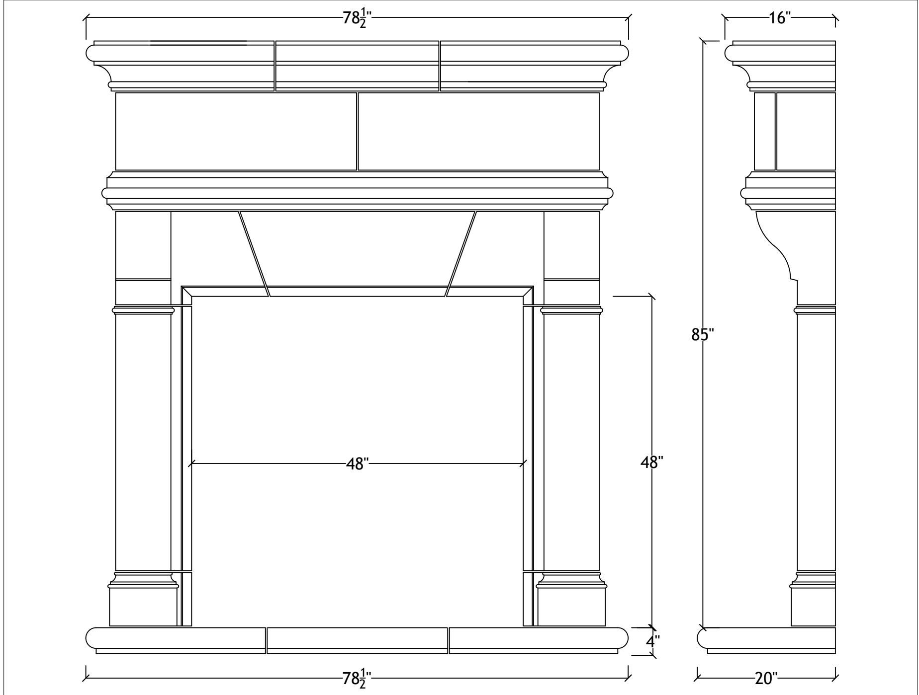
48" Mandalay with bullnosed hearth
