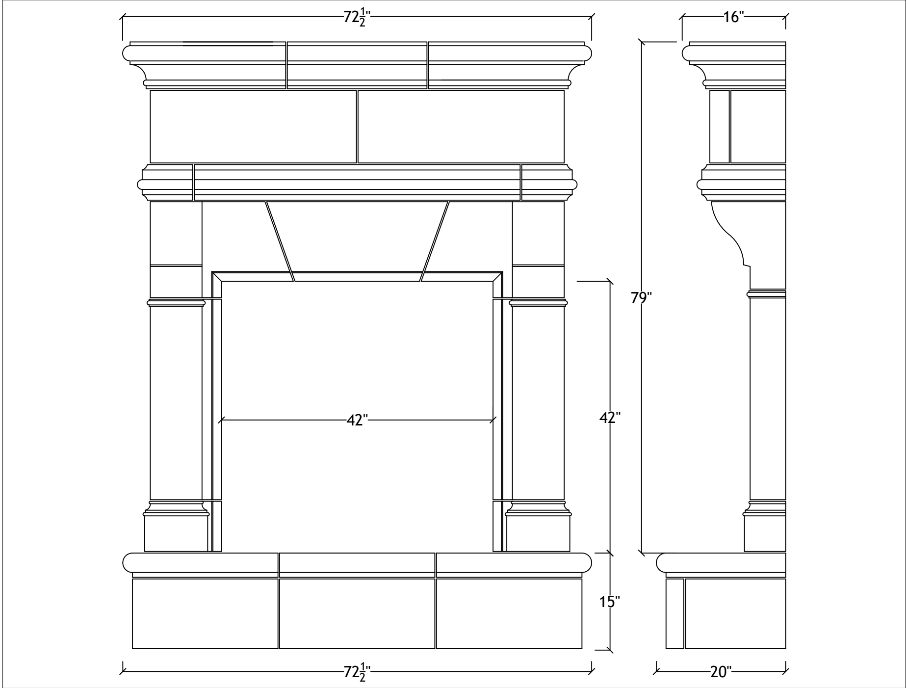
A 1 42" Mandalay with raised bullnosed hearth
