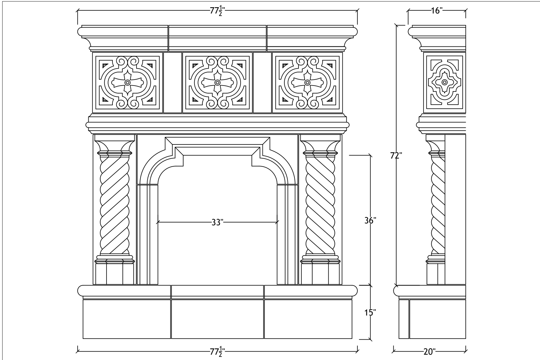
33" Majorca with bullnosed raised hearth
