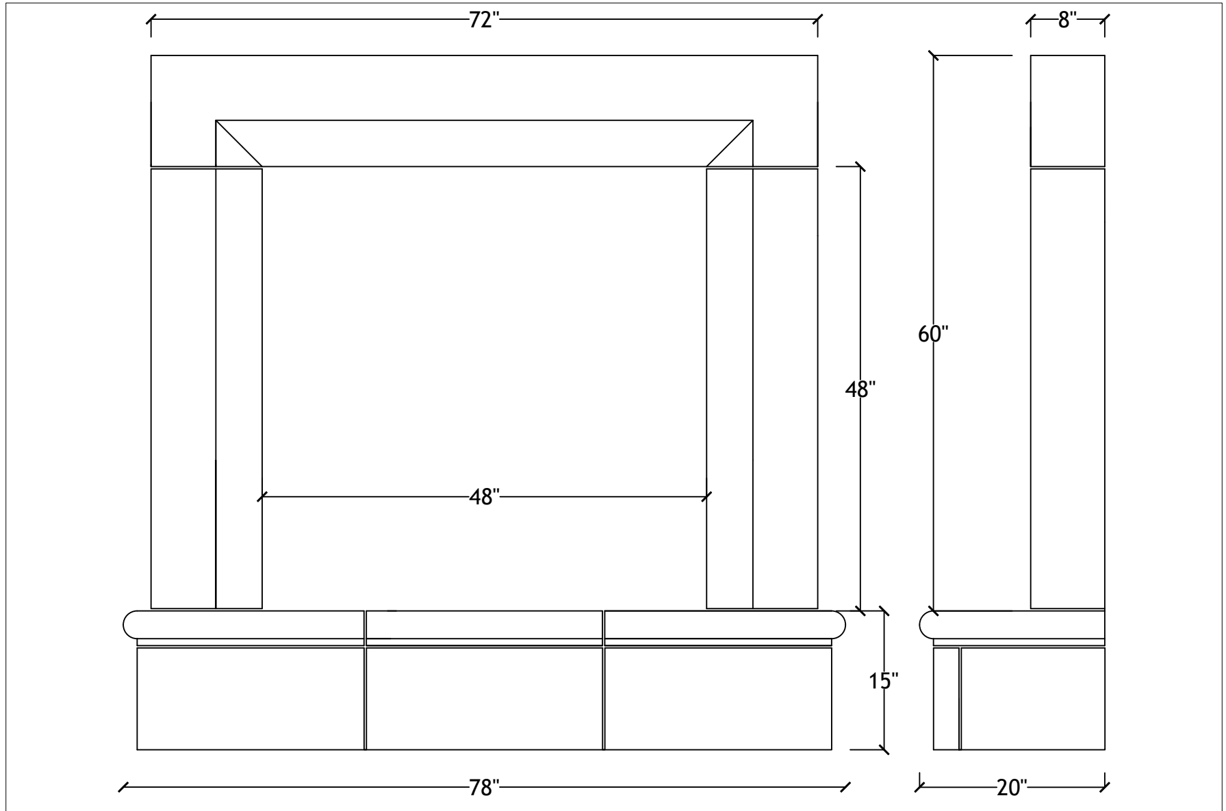
48" Loft with Raised Bullnosed Hearth
