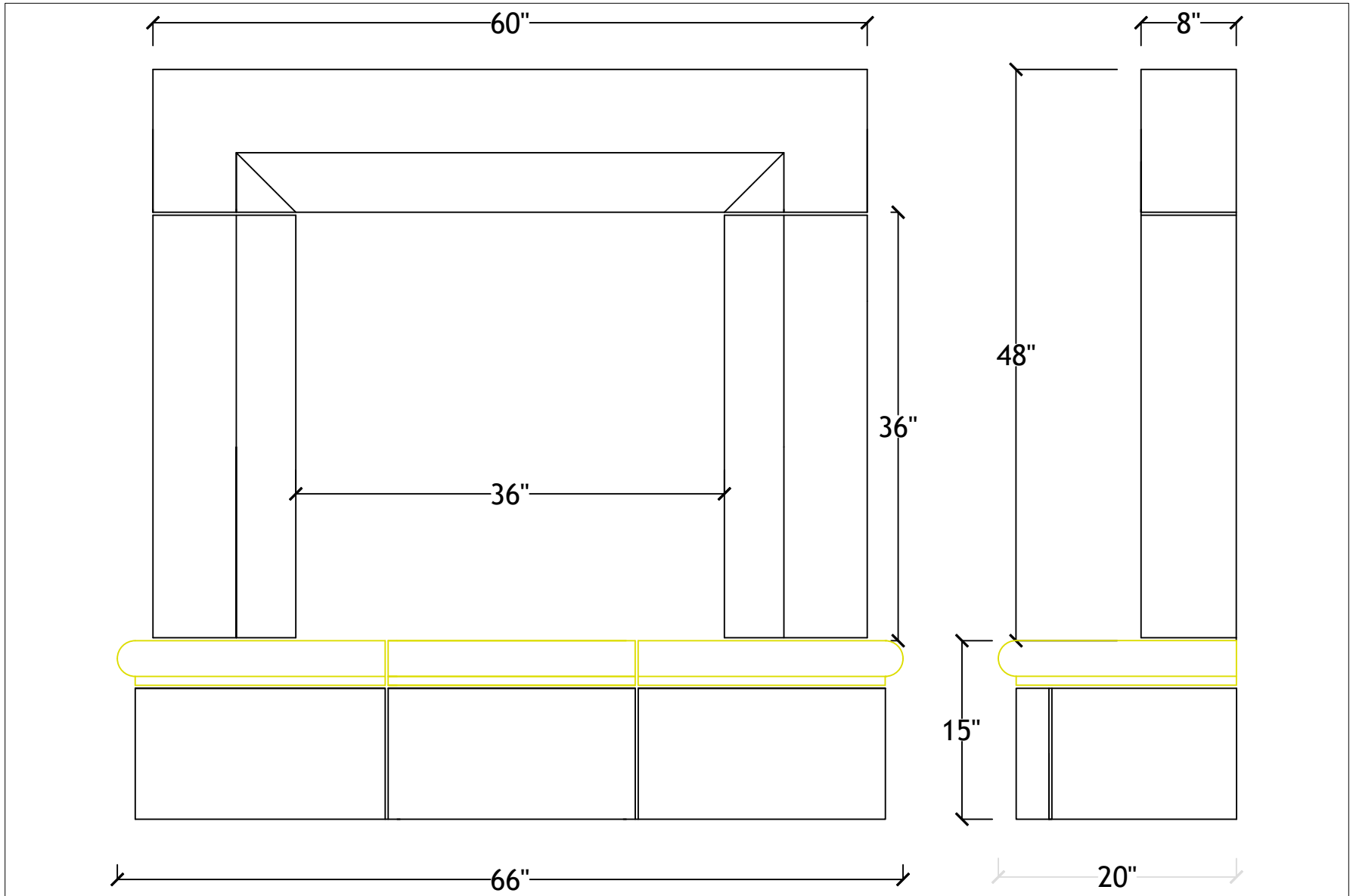
36" Loft with Raised Bullnose Hearth
