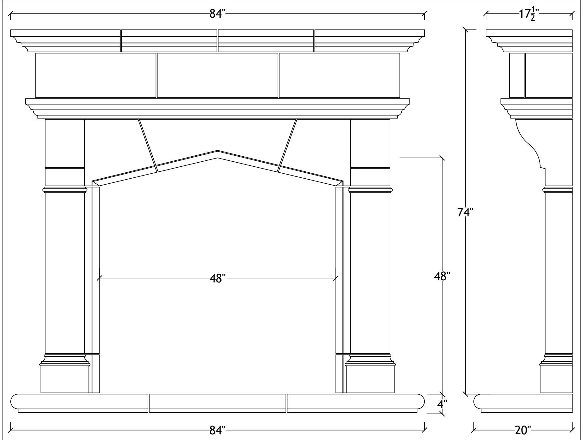
48" Lexington with bullnosed hearth
