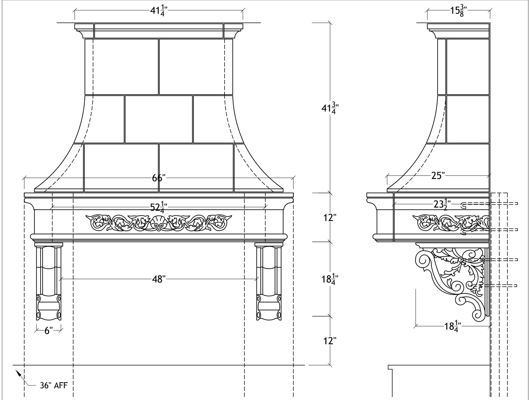
48" Le Petite Range Hood for 10" ceiling
