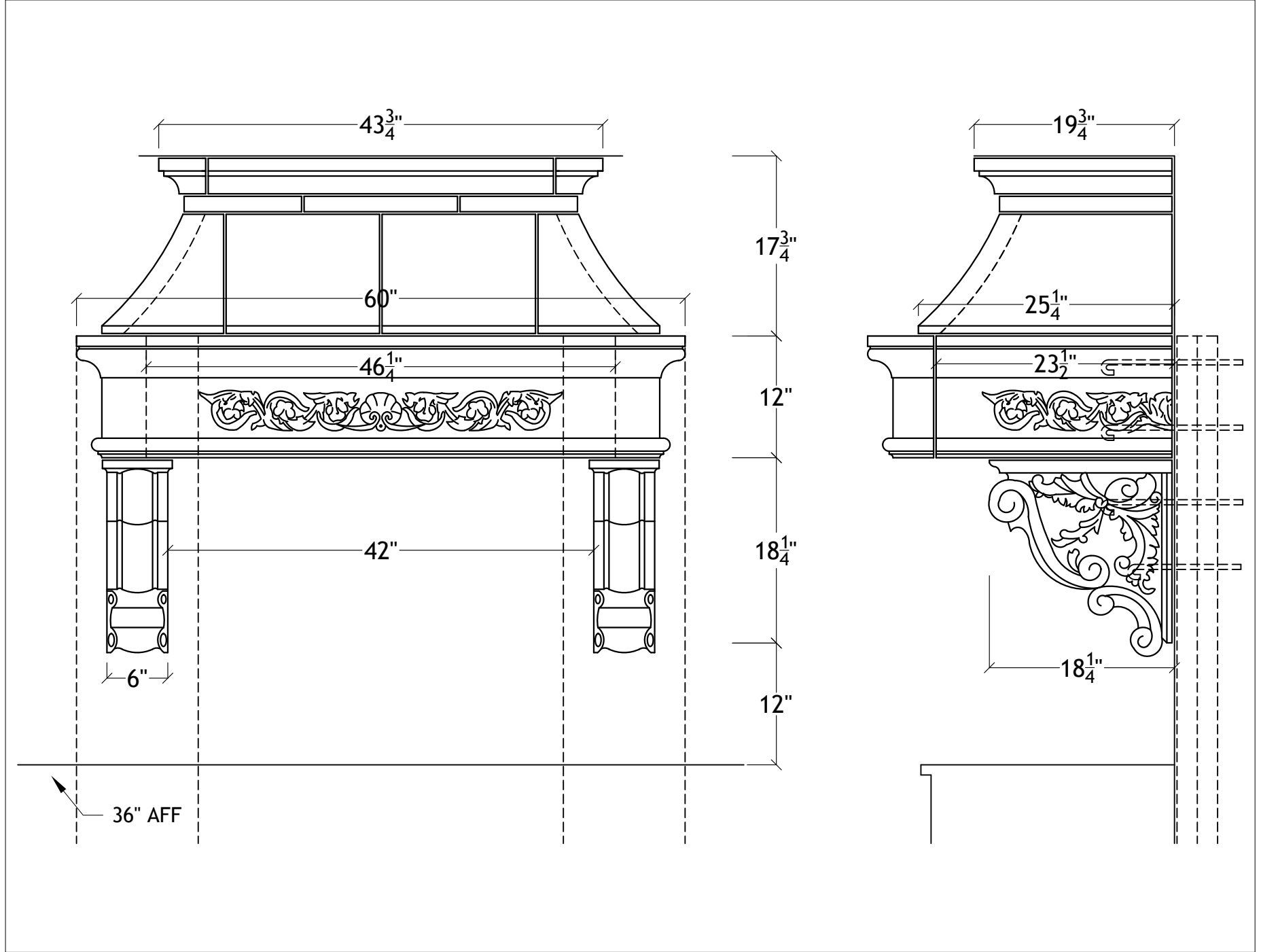
42" Le Petite Range Hood for 8" ceiling
