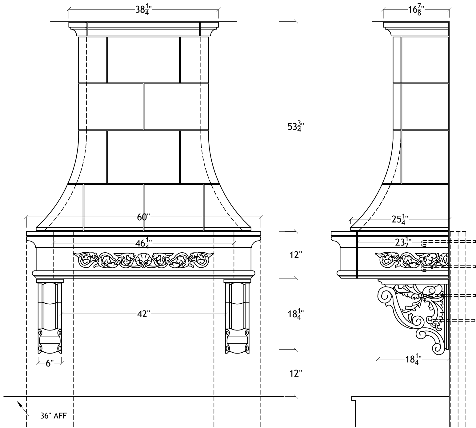
42" Le Petite Range Hood for 11" ceiling
