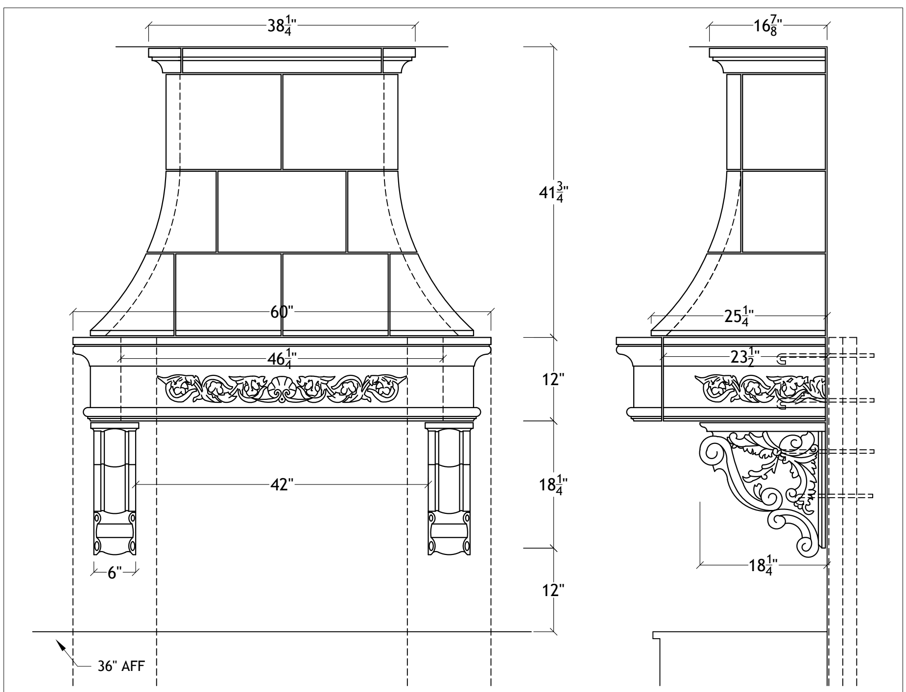
42" Le Petite Range Hood for 10" ceiling
