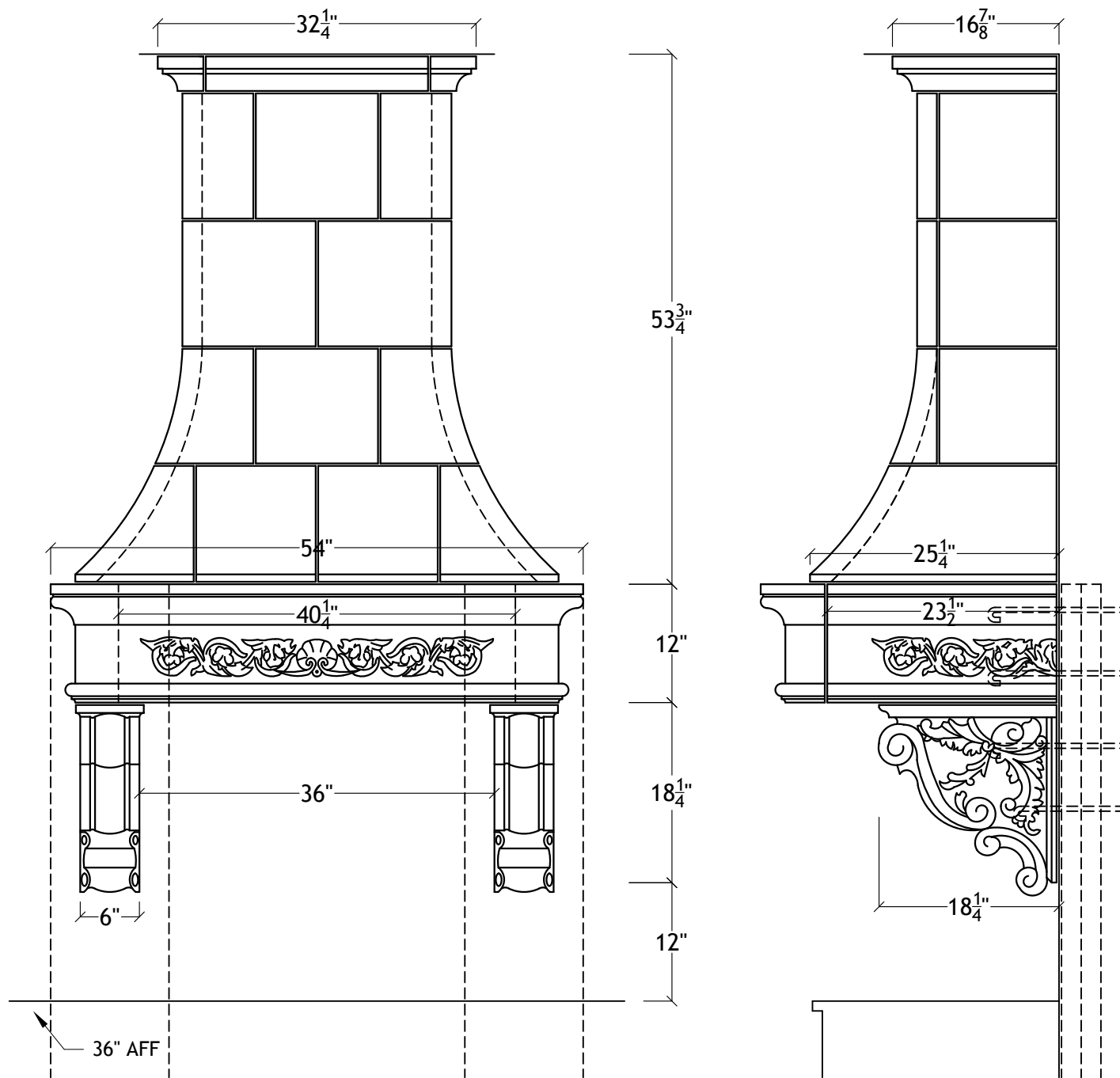
36" Le Petite Range Hood for 11" ceiling
