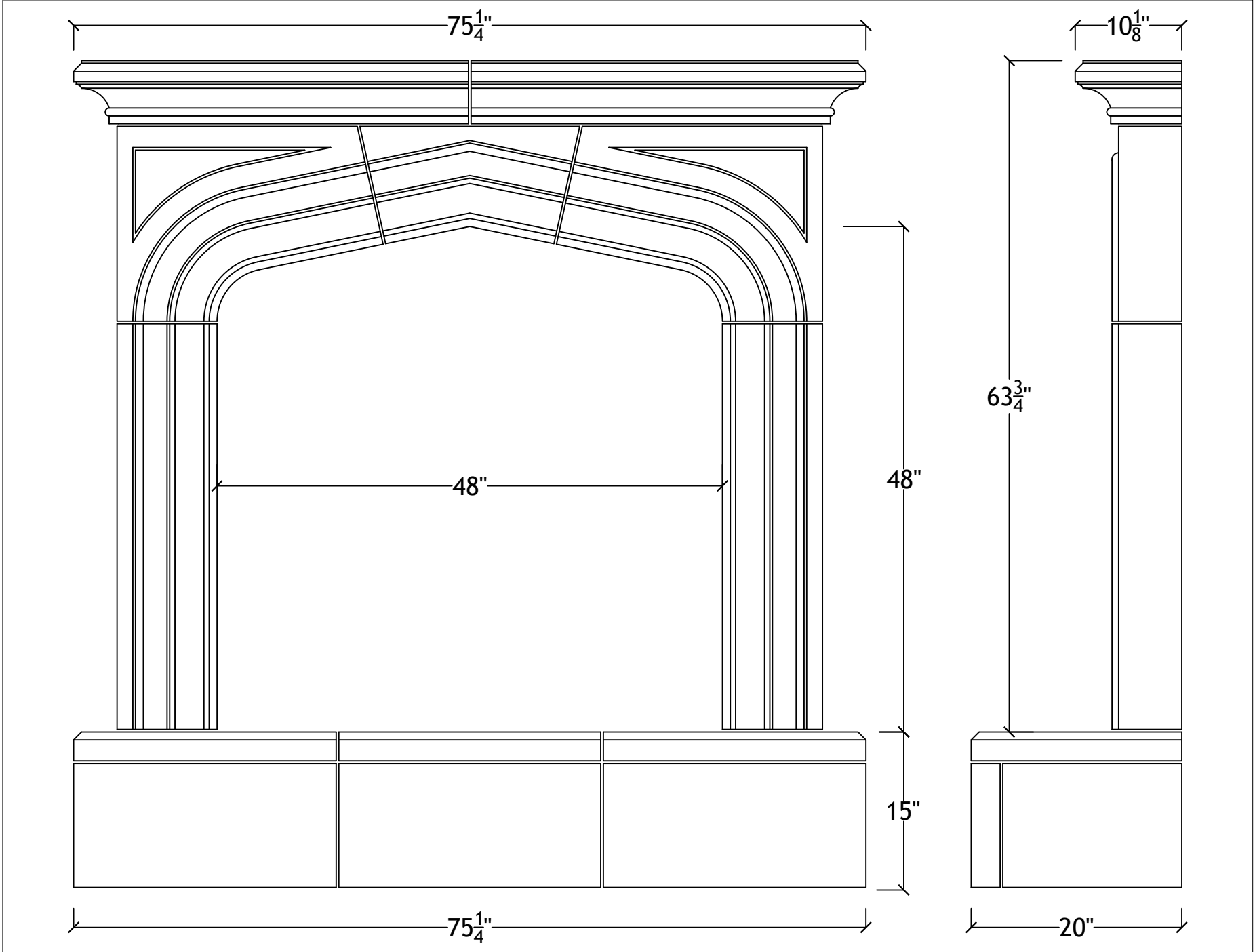
48" Laurent with raised hearth
