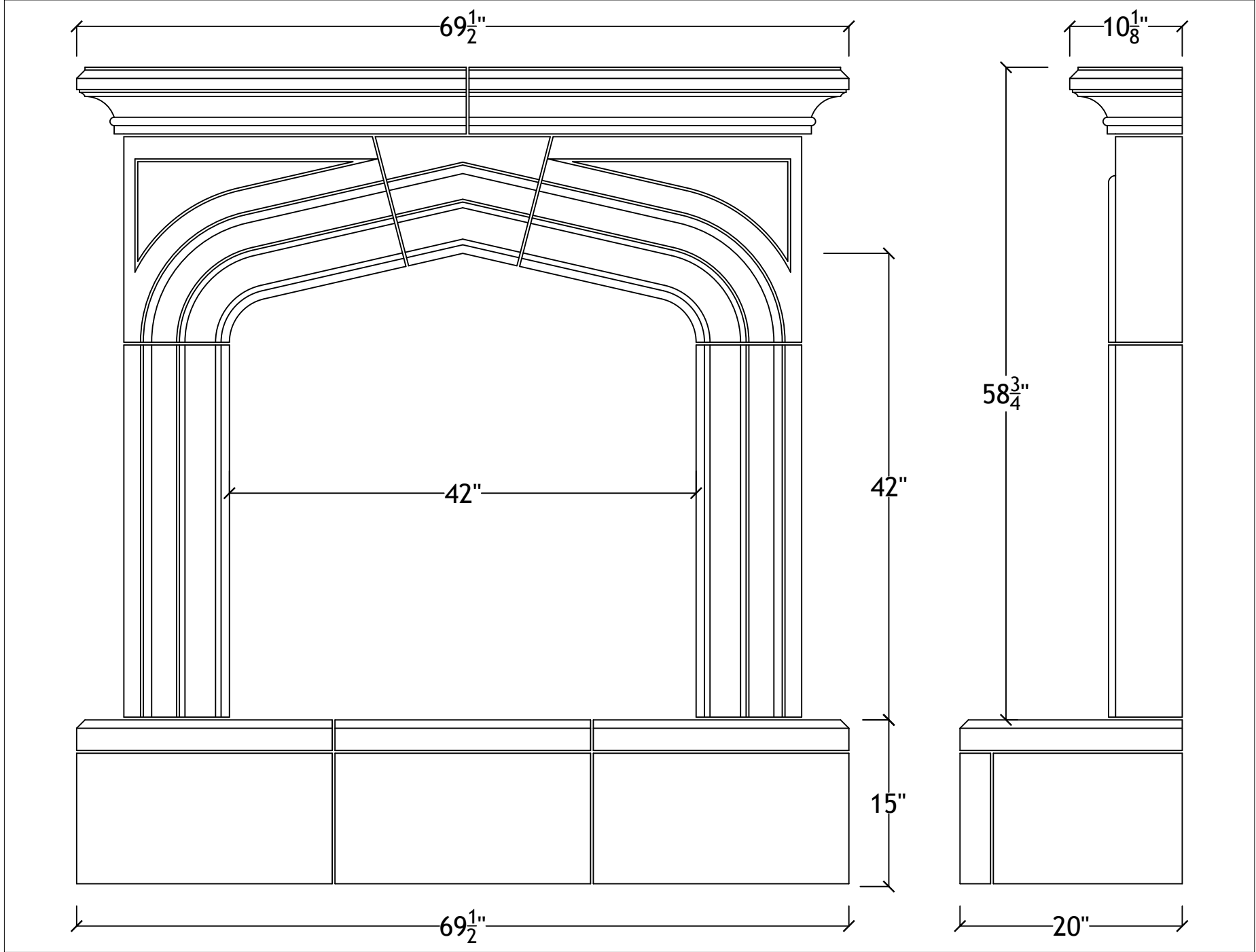
42" Laurent with raised hearth
