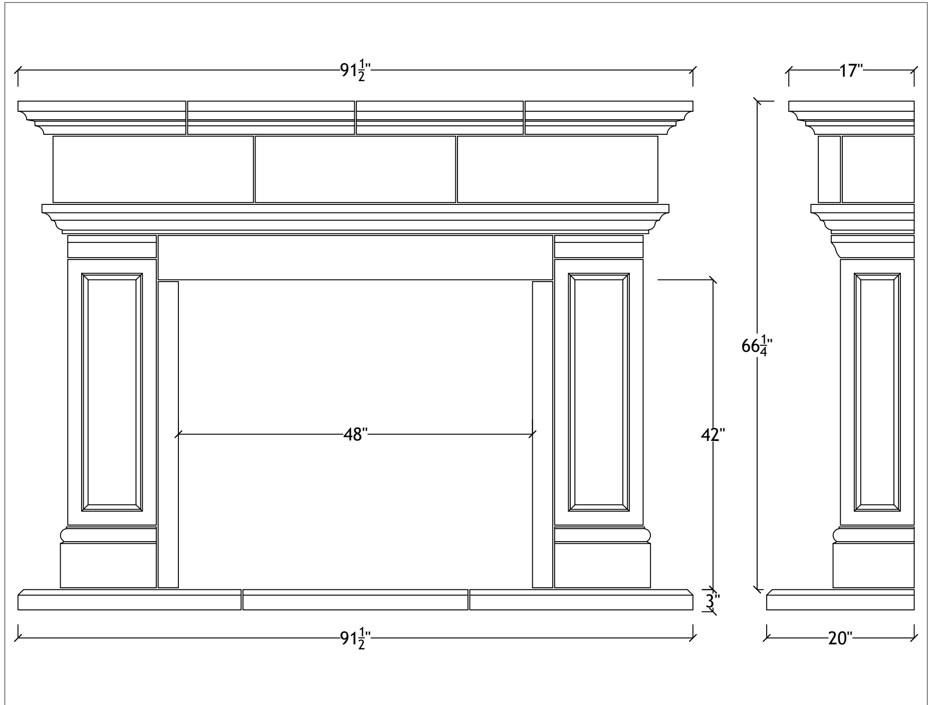
48" Hampton with hearth
