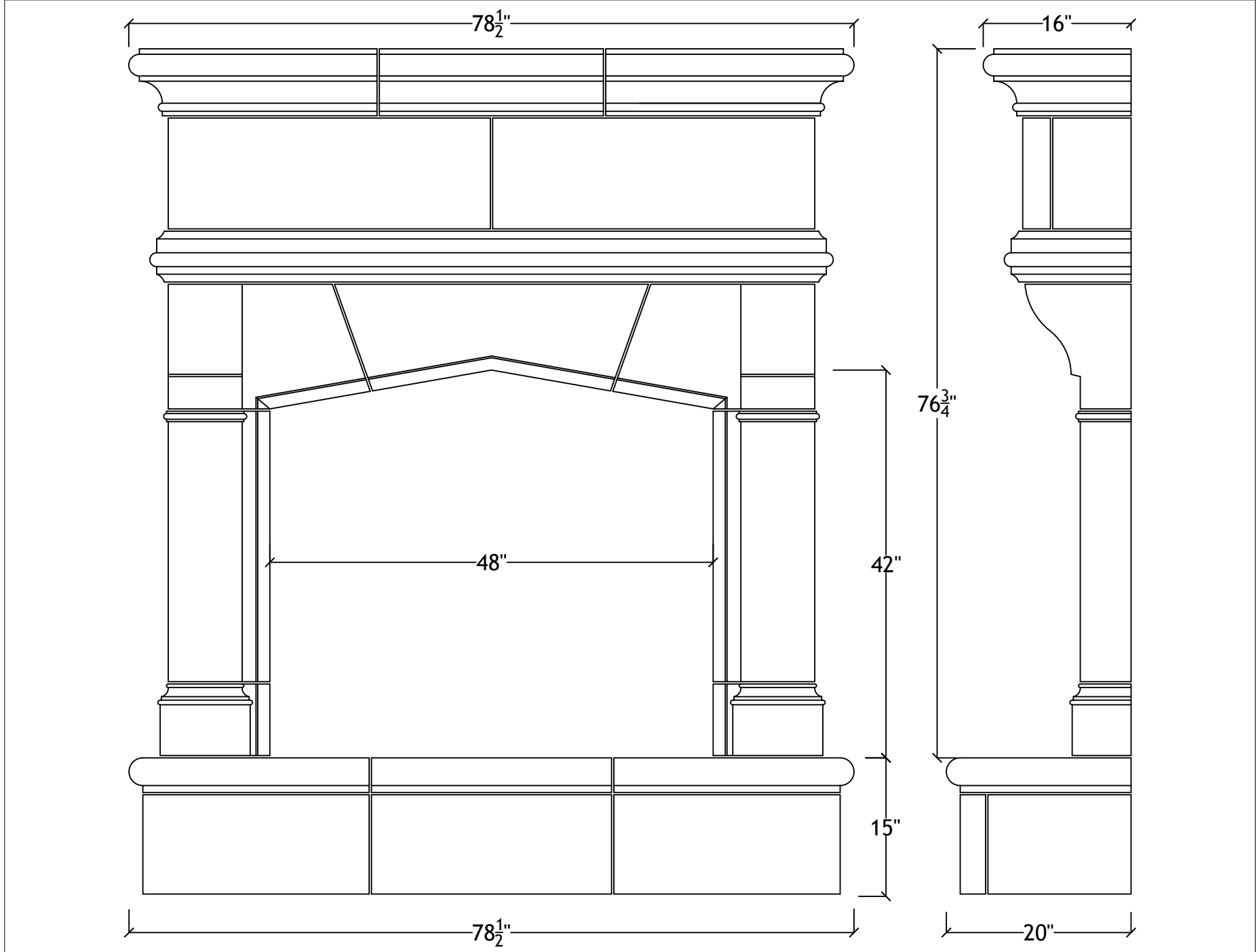
48" Gatwick with raised bullnosed hearth
