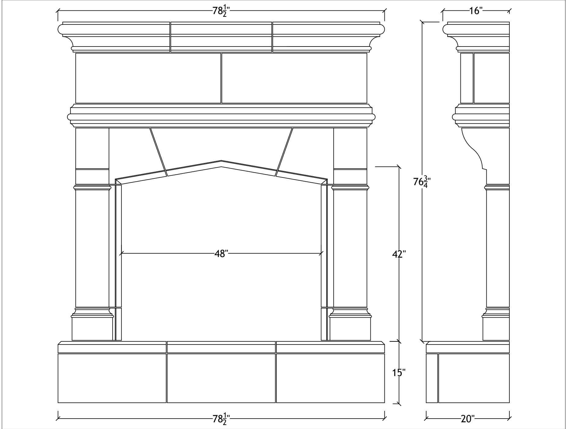
48" Gatwick with raised hearth
