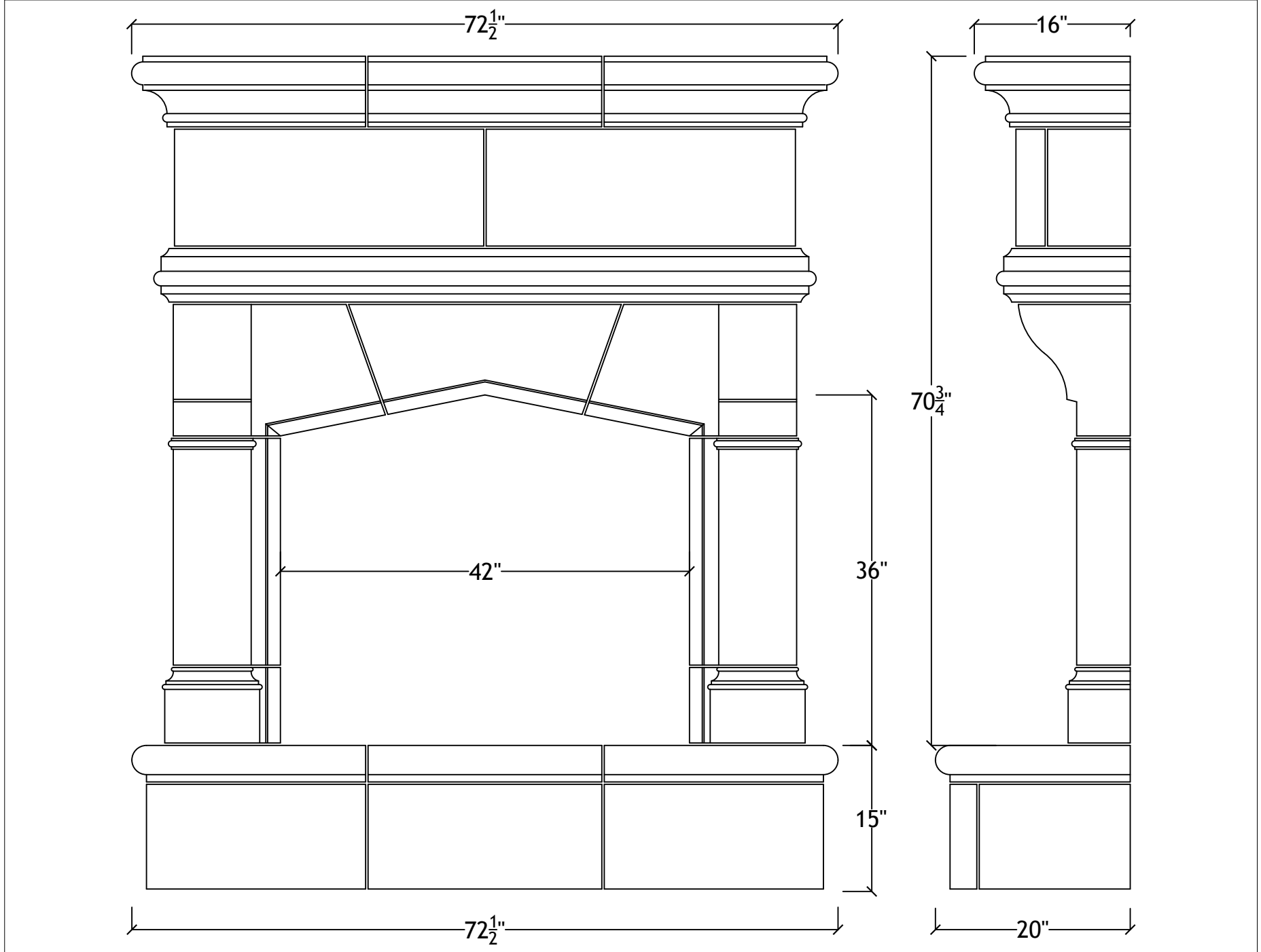
42" Gatwick with raised bullnosed hearth
