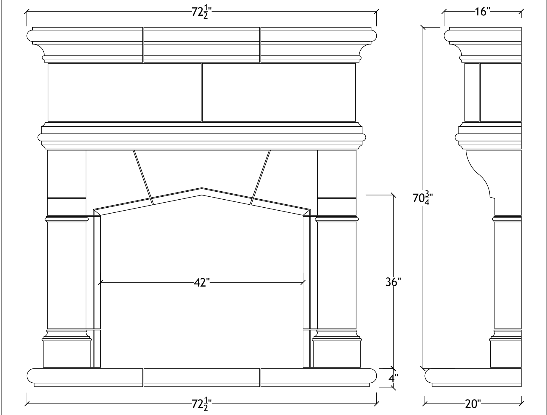
42" Gatwick with bullnosed hearth
