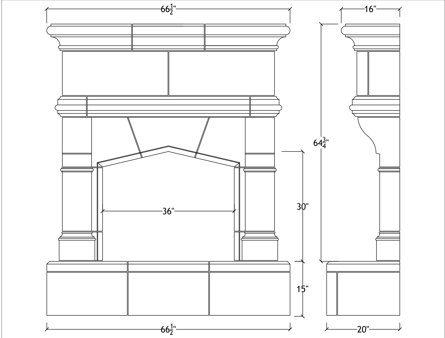
36" Gatwick with raised hearth
