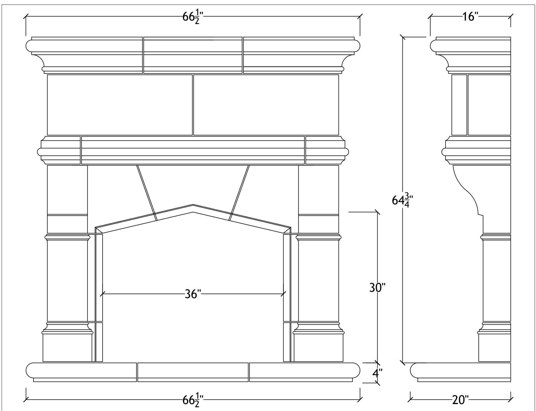
36" Gatwick with bullnosed hearth
