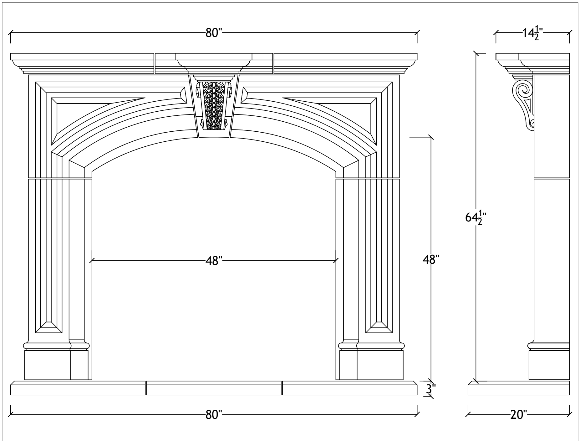
48" Fremont with hearth
