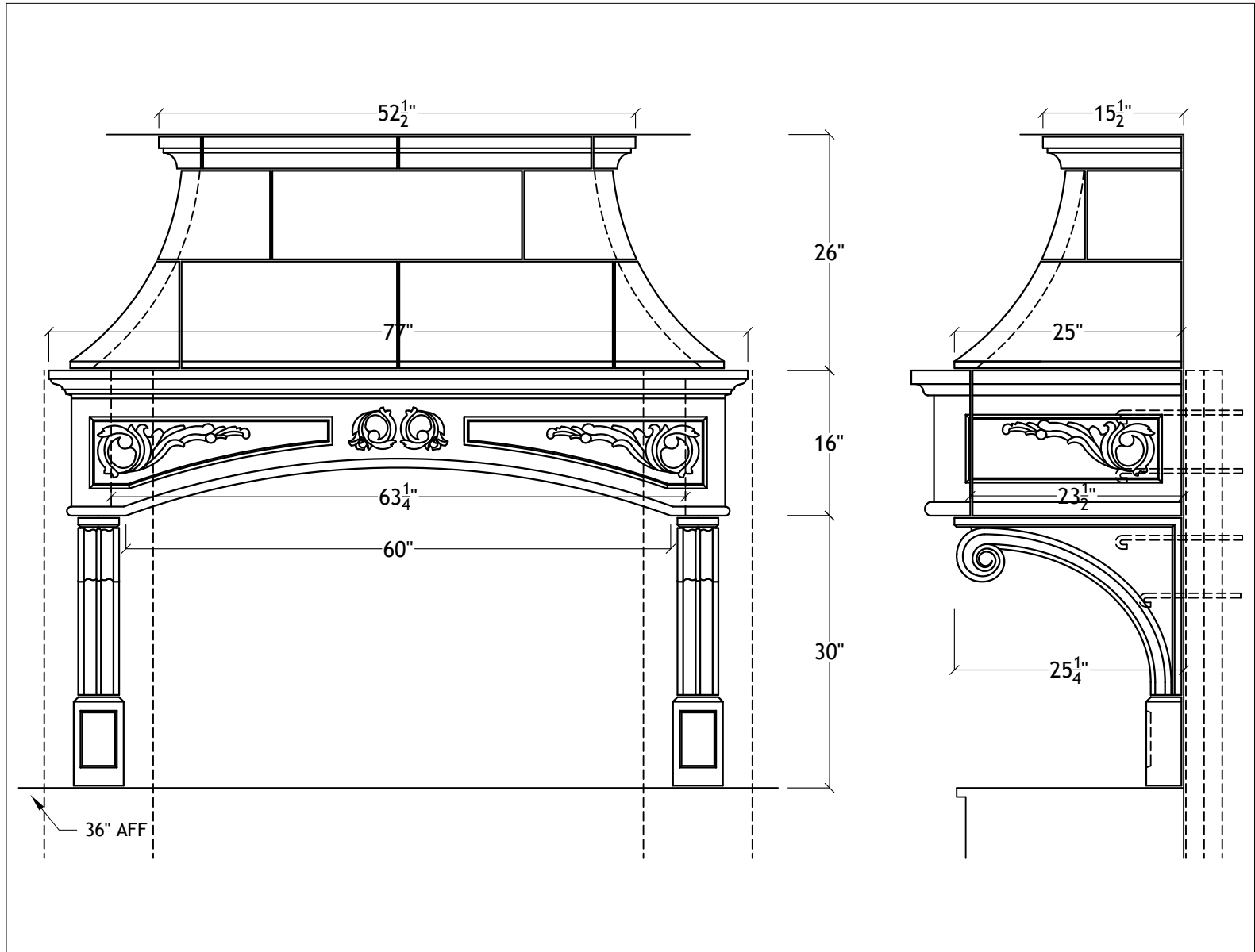
60" Florentine Range Hood for 9' ceiling
