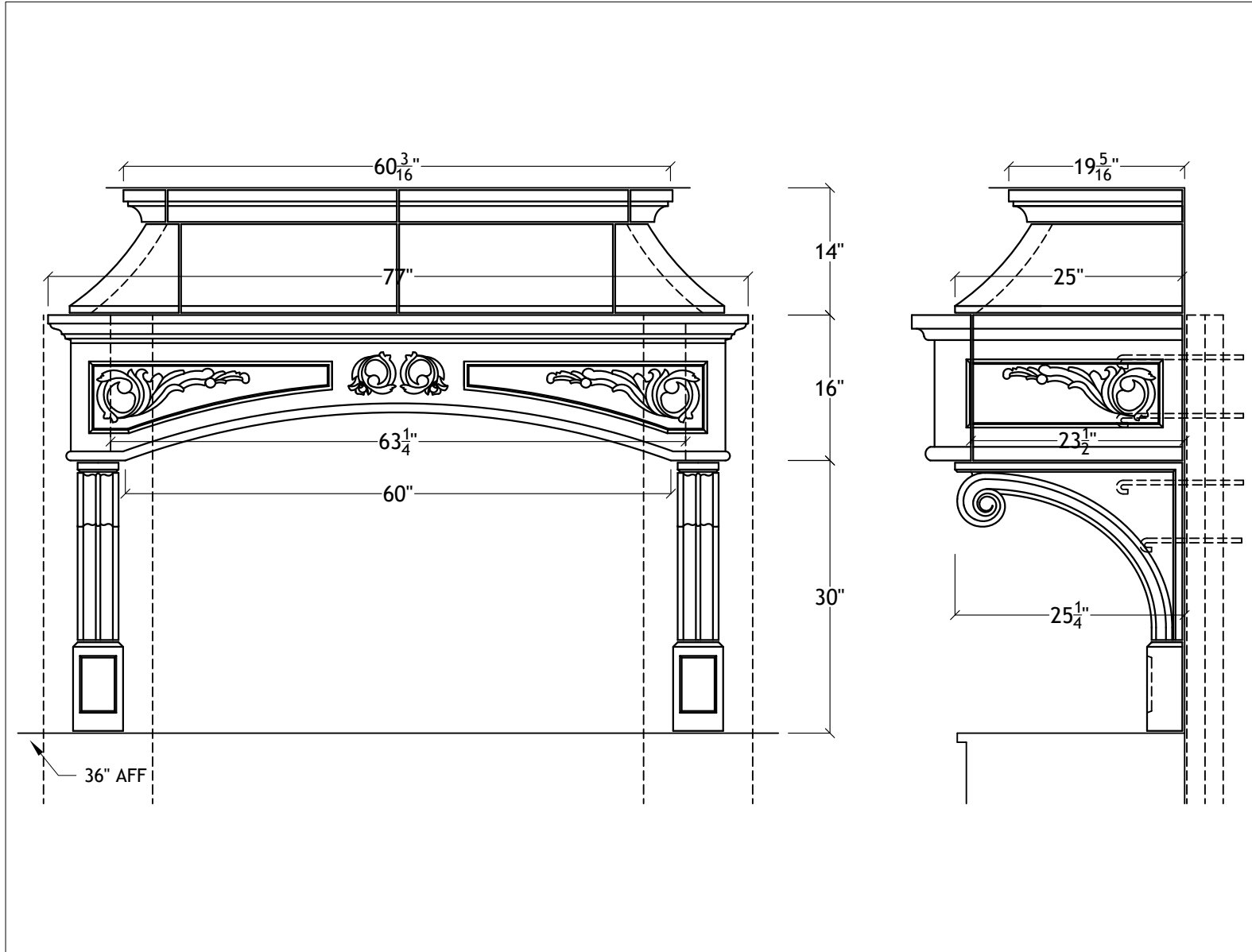
60" Florentine Range Hood for 8' ceiling
