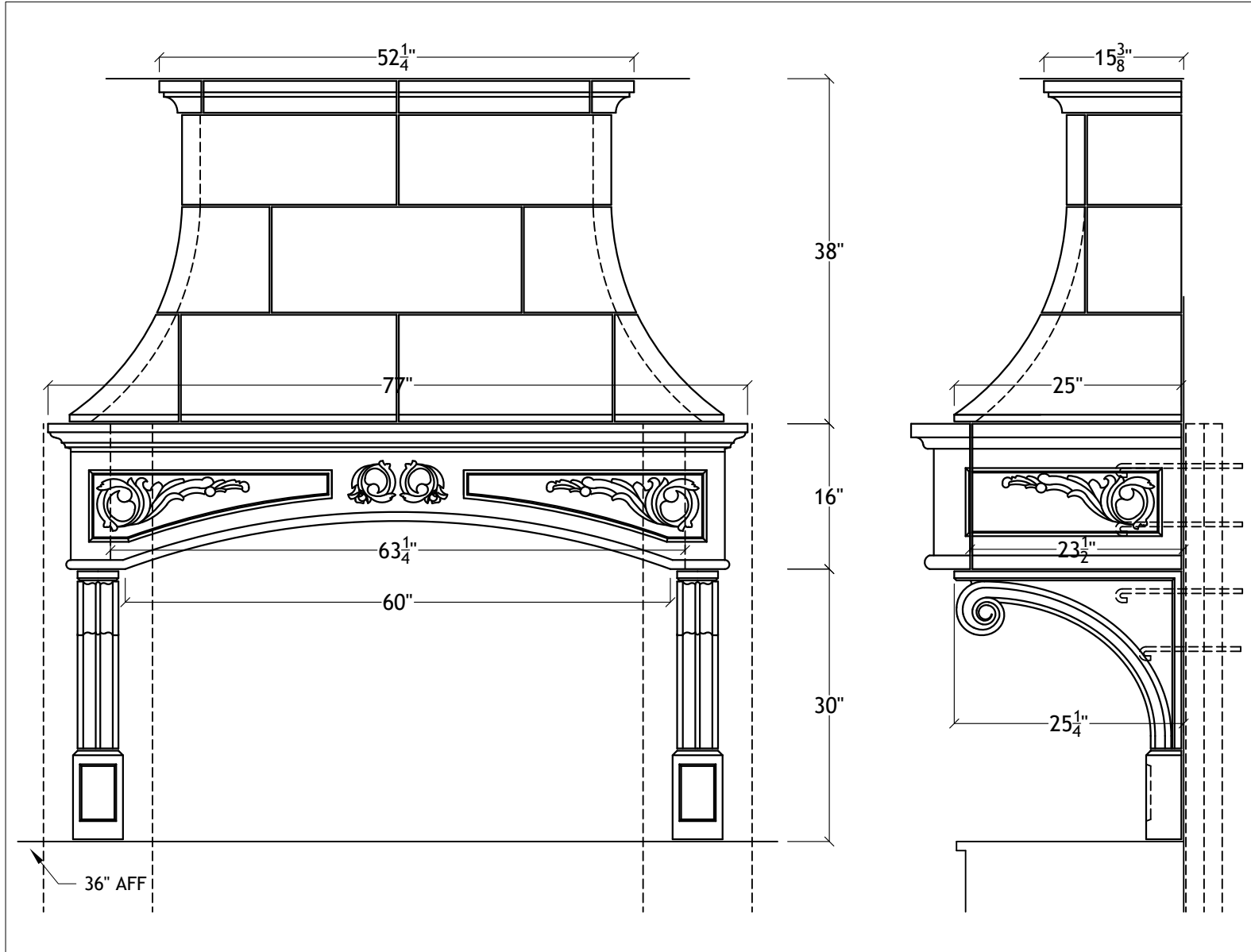
60" Florentine Range Hood for 10' ceiling
