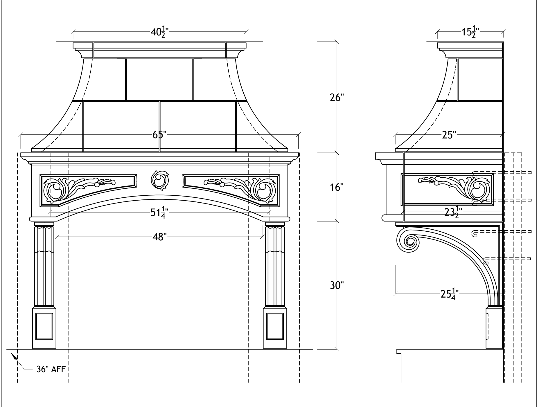
48" Florentine Range Hood for 9' ceiling
