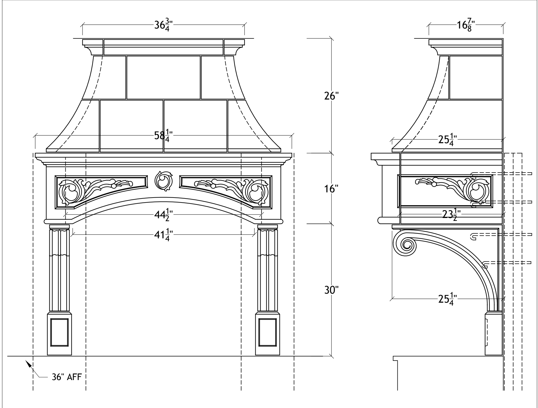
42" Florentine Range Hood for 9' ceiling
