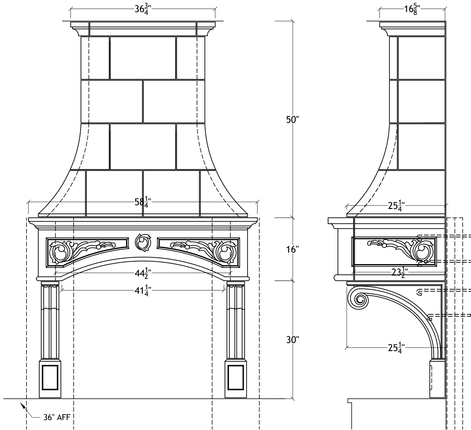
42" Florentine Range Hood for 11' ceiling
