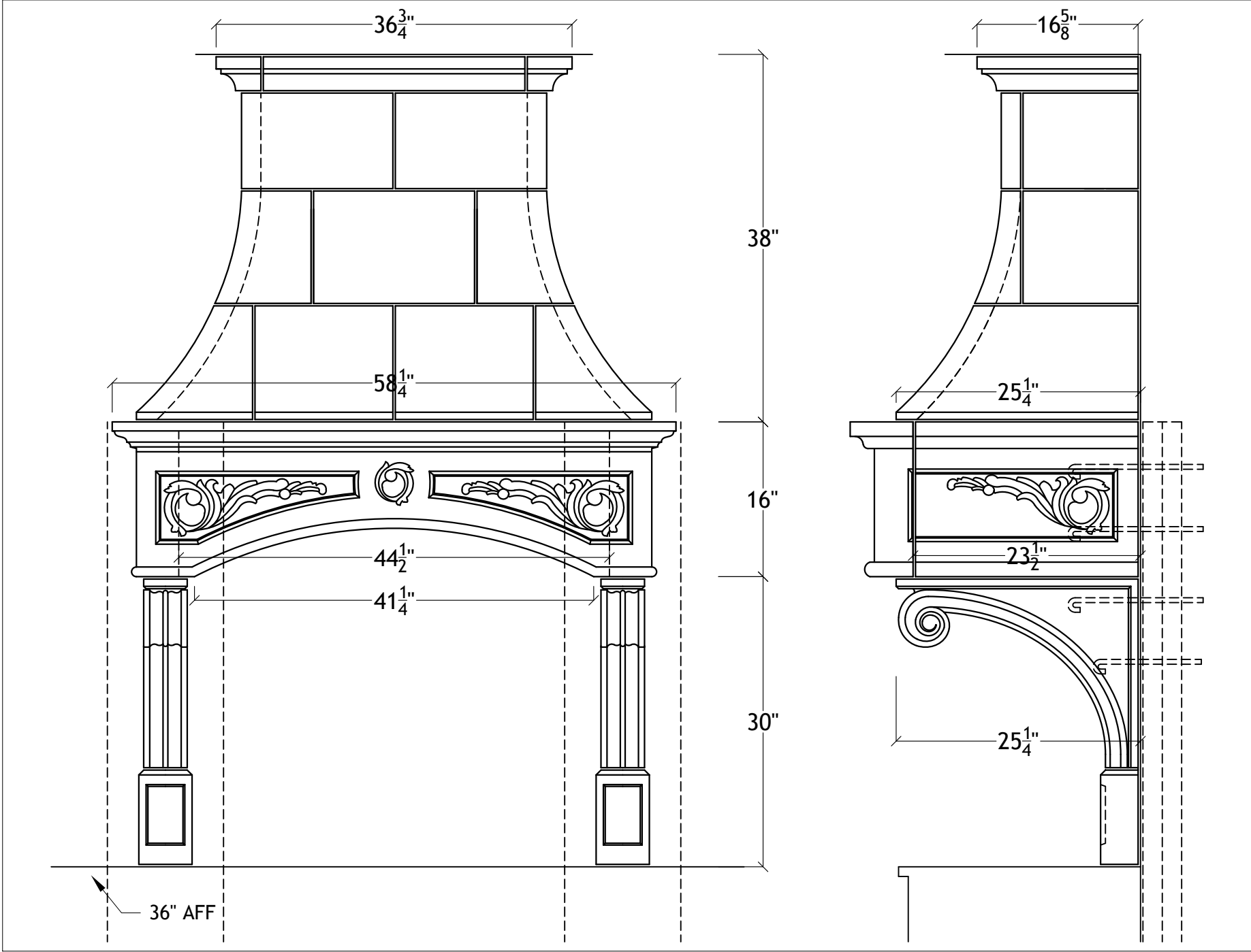
42" Florentine Range Hood for 10' ceiling
