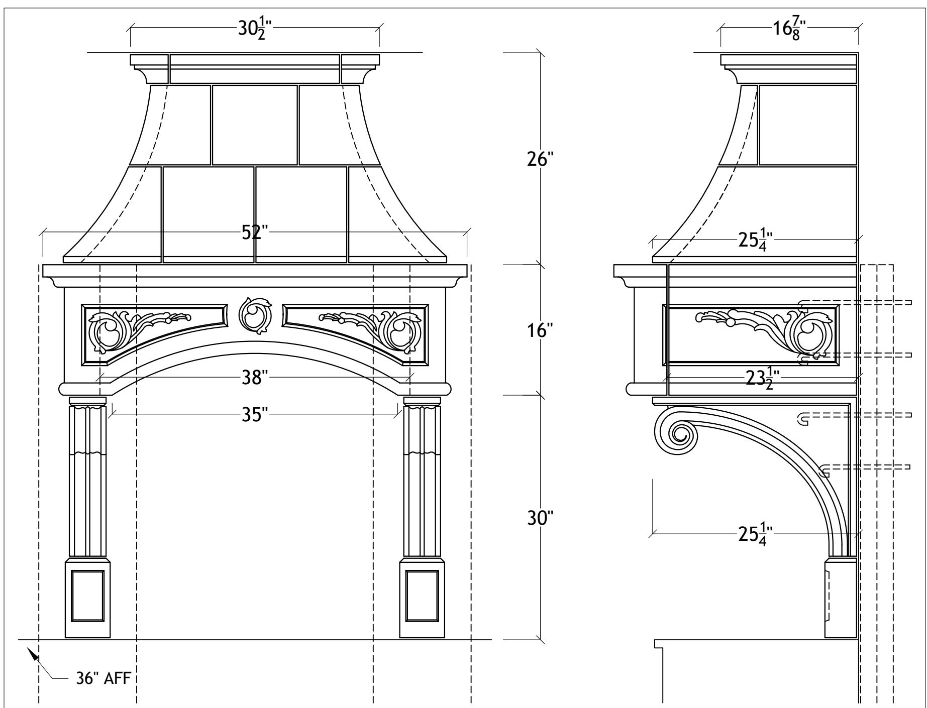
36" Florentine Range Hood for 9' ceiling
