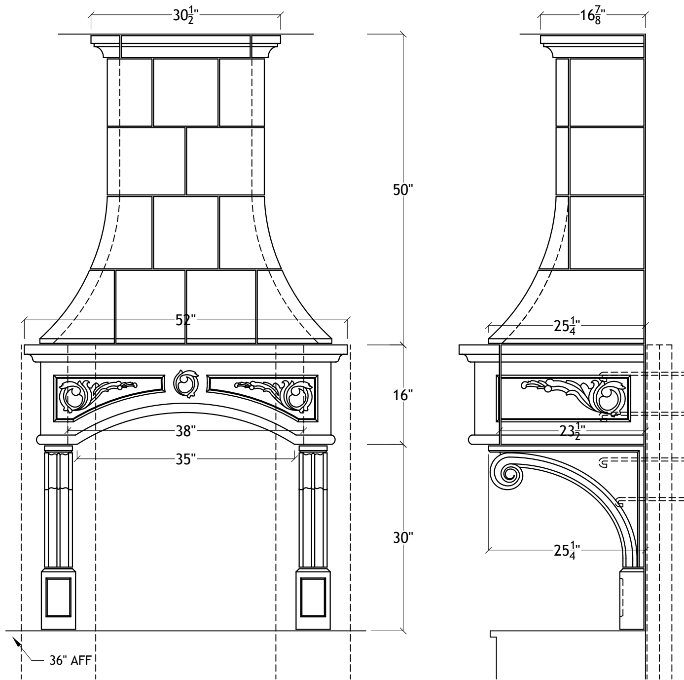
36" Florentine Range Hood for 11' ceiling
