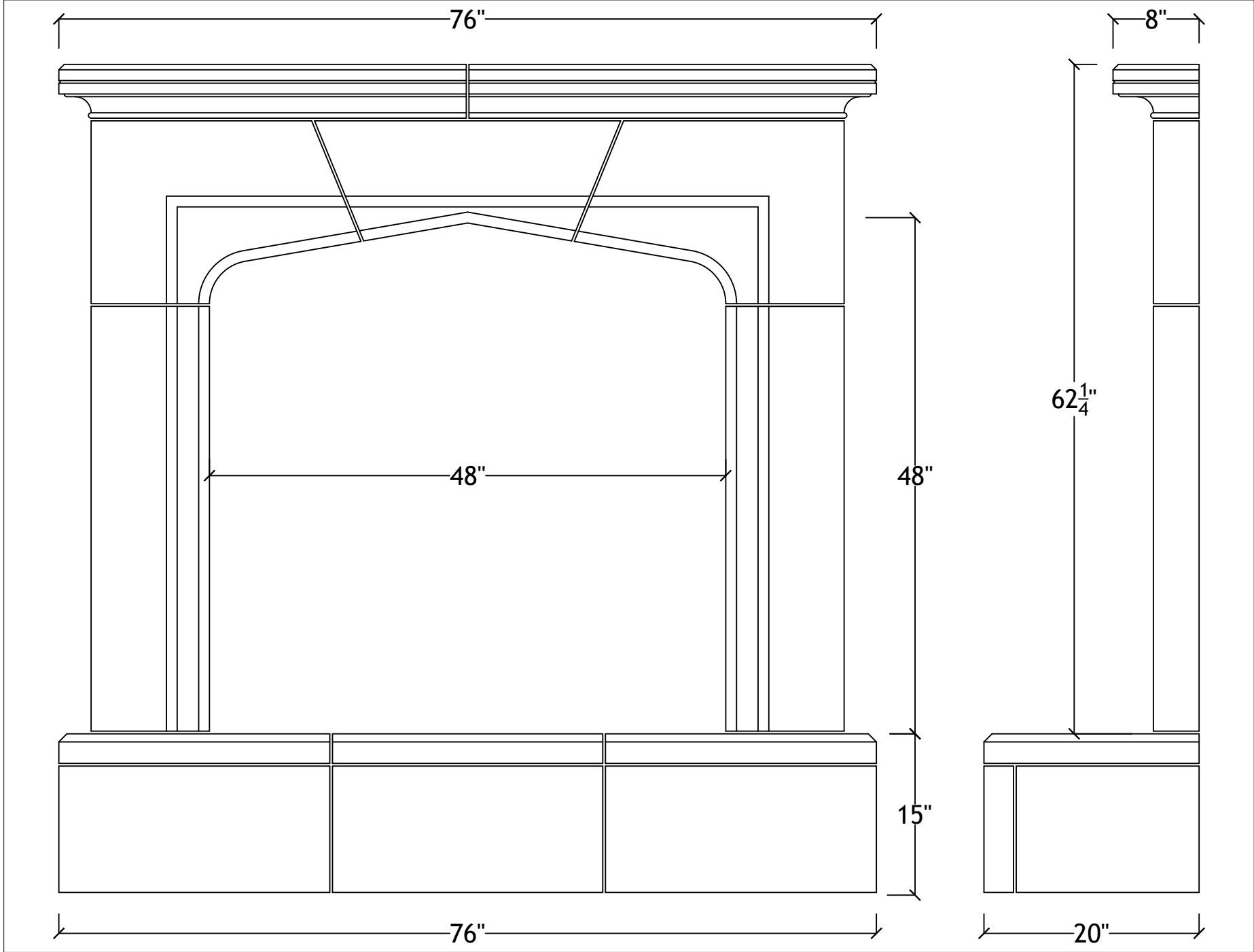
48" Fairmount with raised hearth
