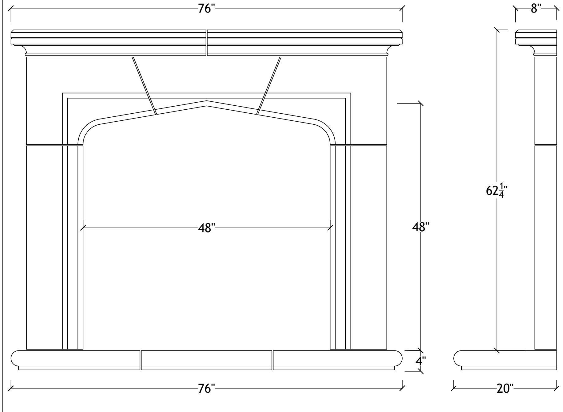
48" Fairmount with bullnosed hearth
