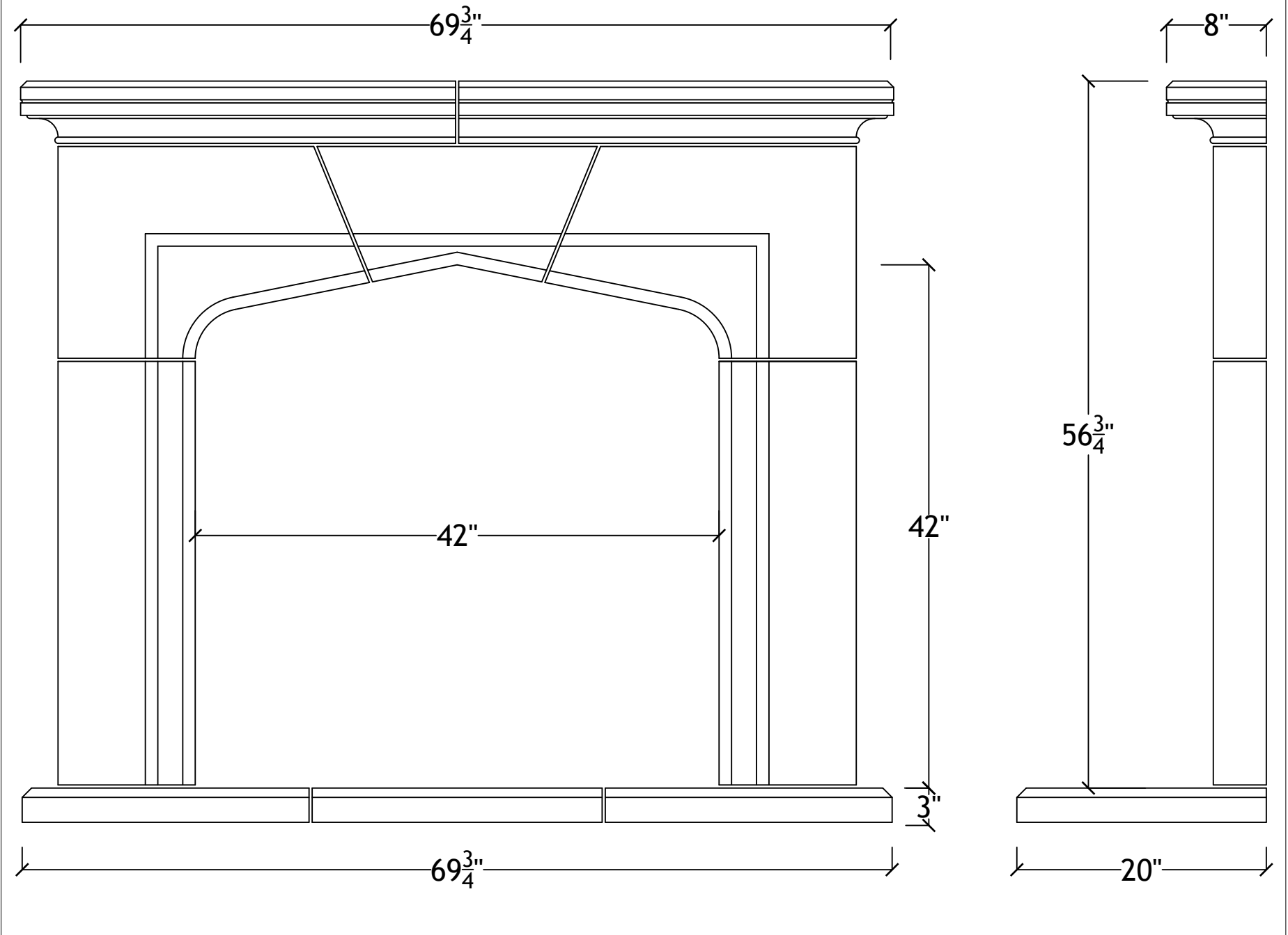
42" Fairmount with hearth
