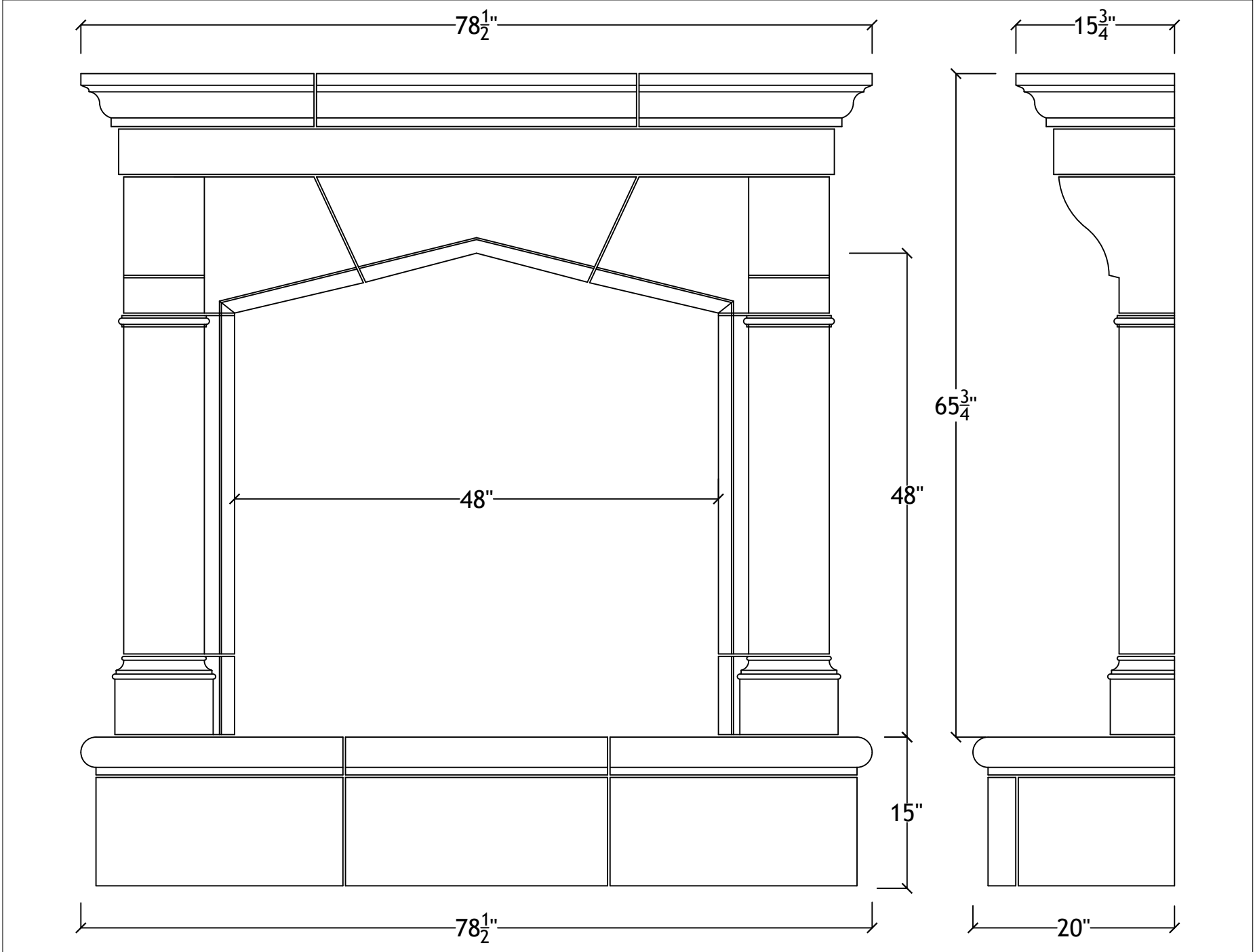
48" Essex with raised bullnosed hearth
