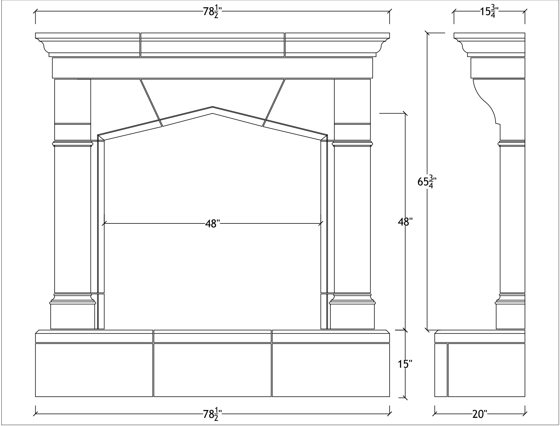
48" Essex with raised hearth
