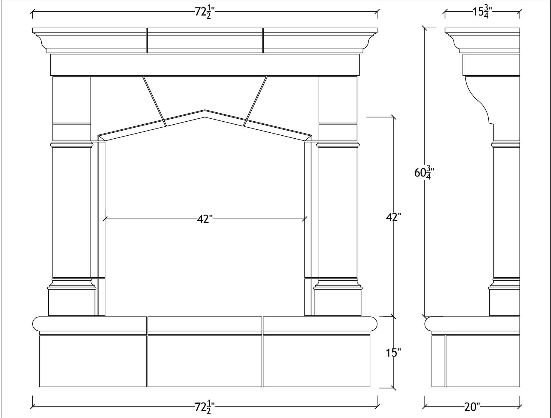
42" Essex with raised bullnosed hearth
