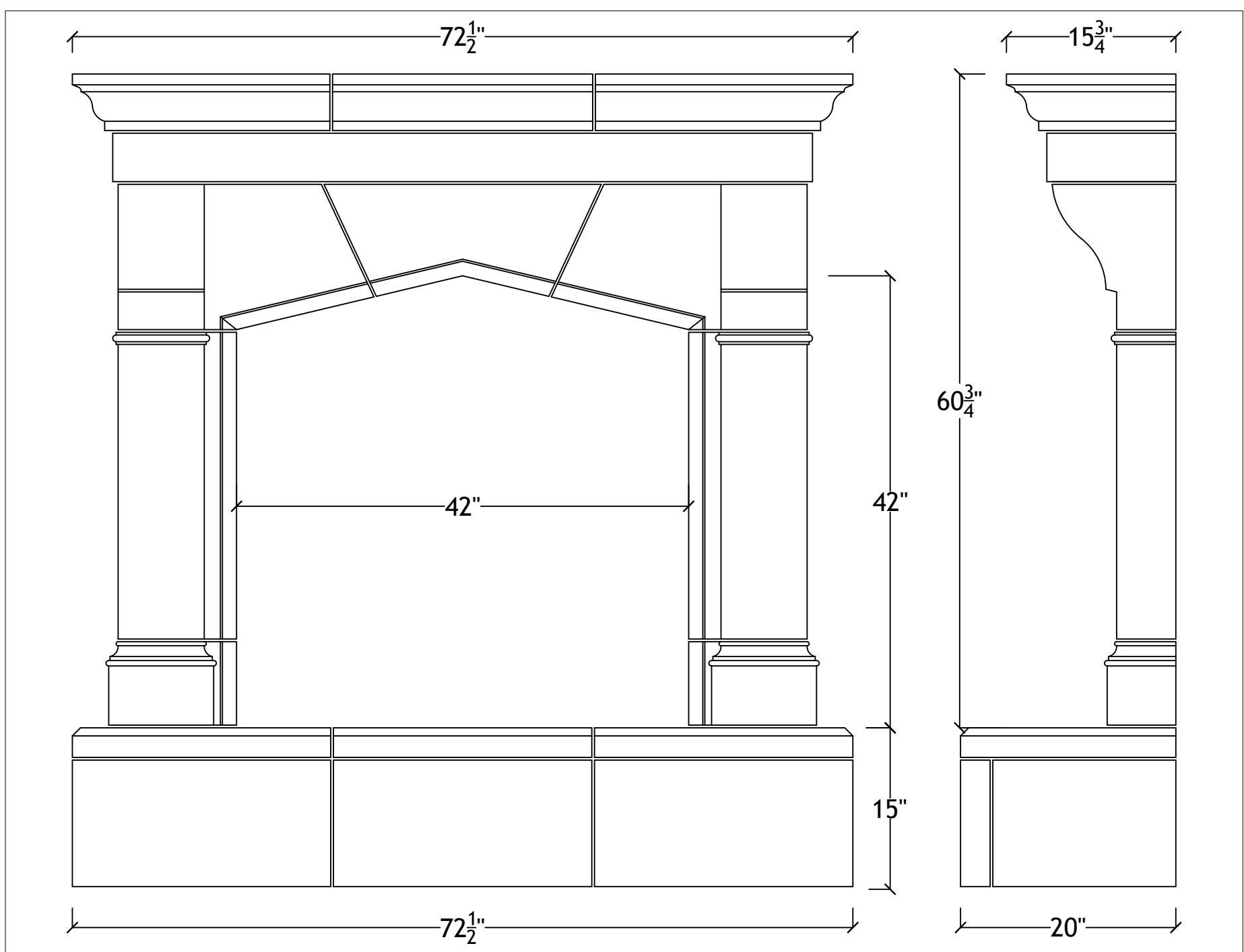
42" Essex with raised hearth
