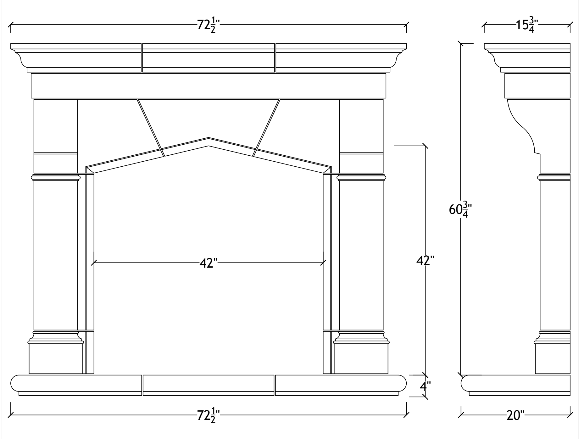
42" Essex with bullnosed hearth
