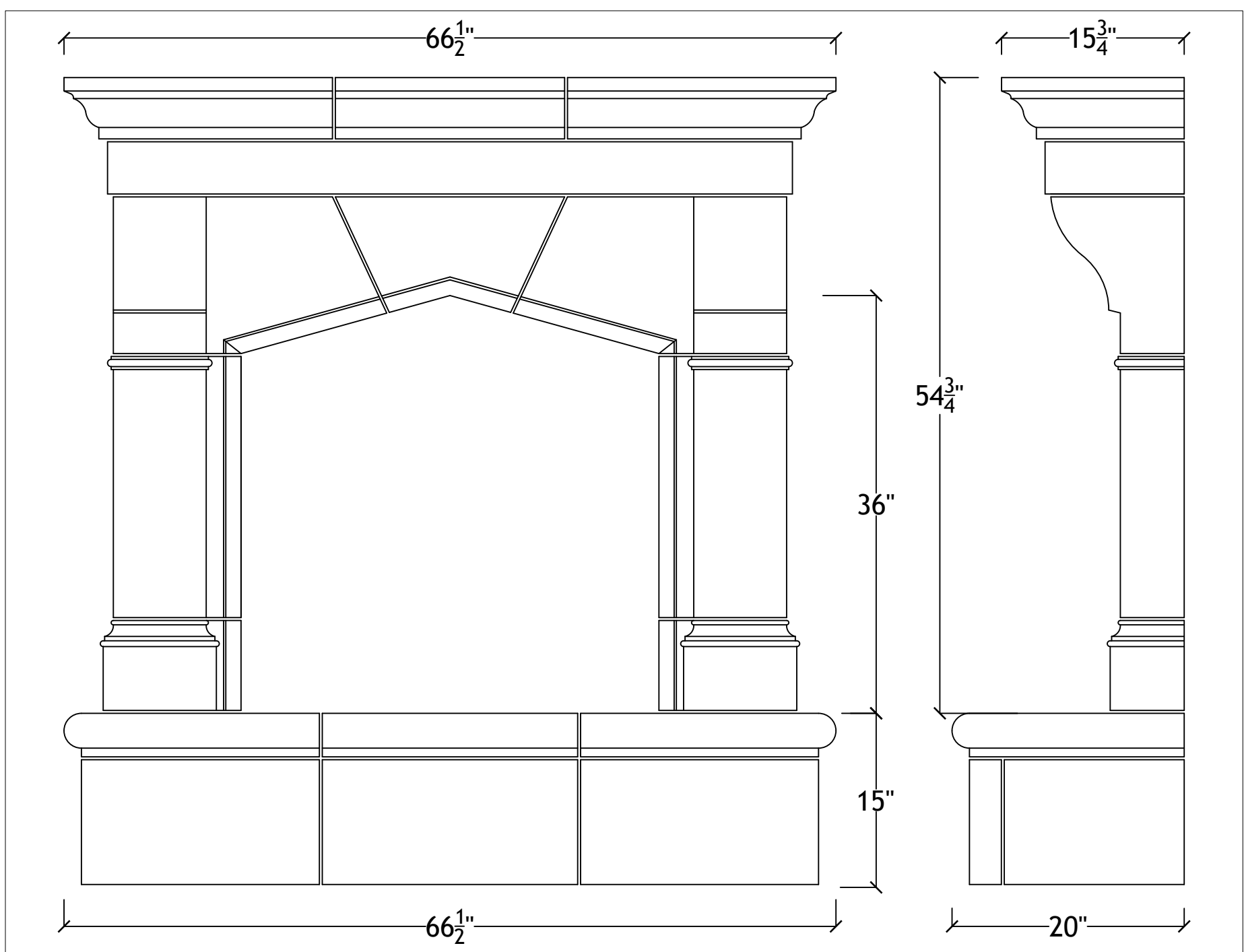
36" Essex with raised bullnosed hearth
